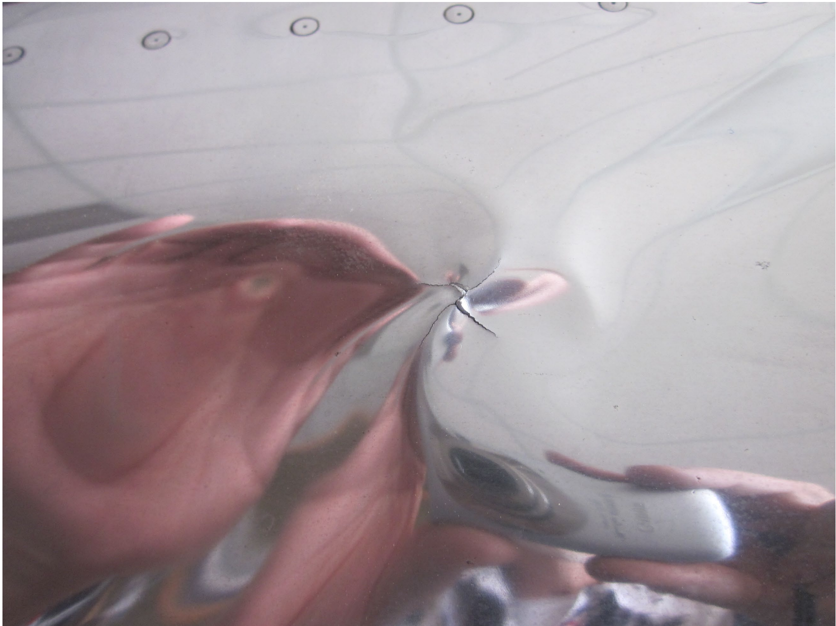
Photo 3 – X Pattern Skin Fracture (FAA Photo)
