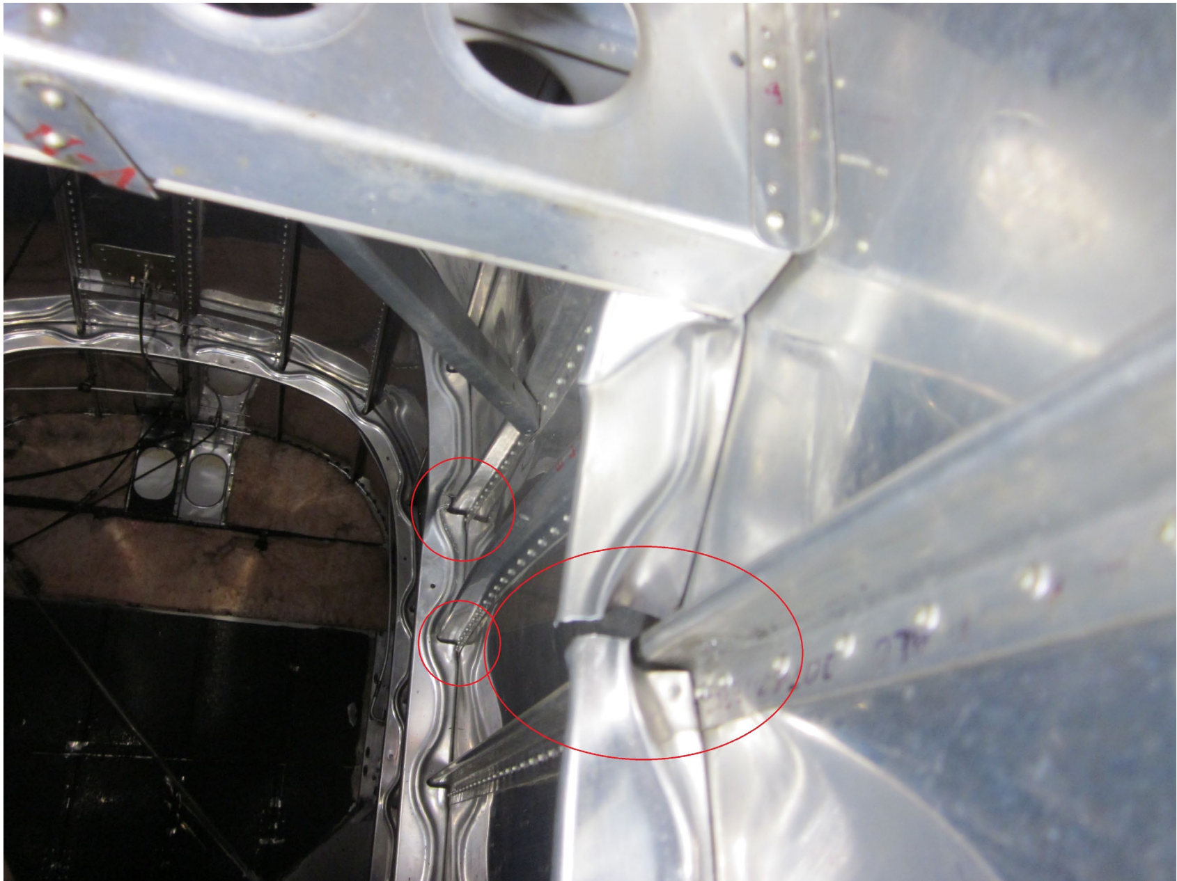
Photo 5 – Damaged 205 and 232 Bulkheads (FAA Photo)
