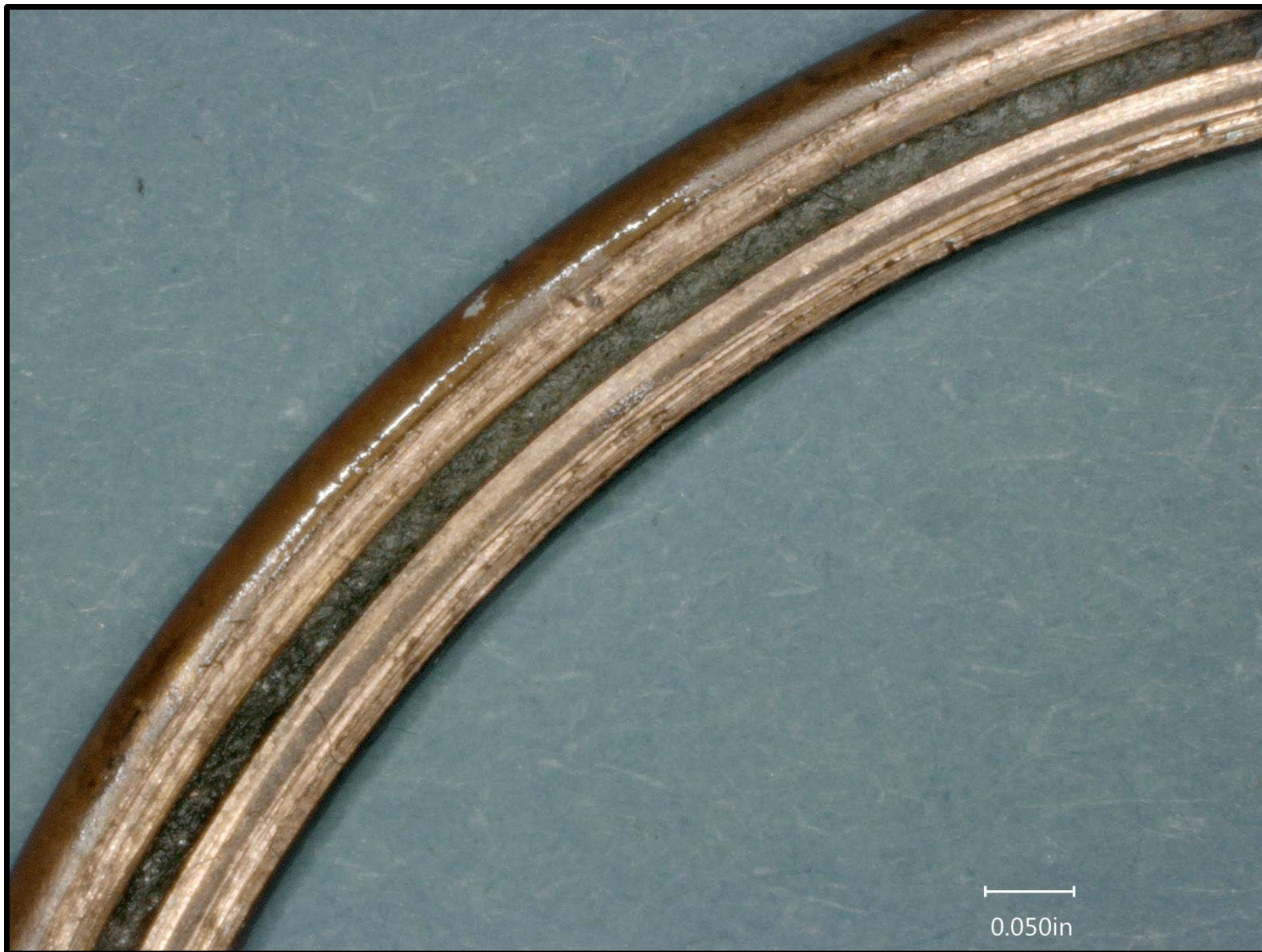
Figure 3: Copper Gasket (portion showing crush)
