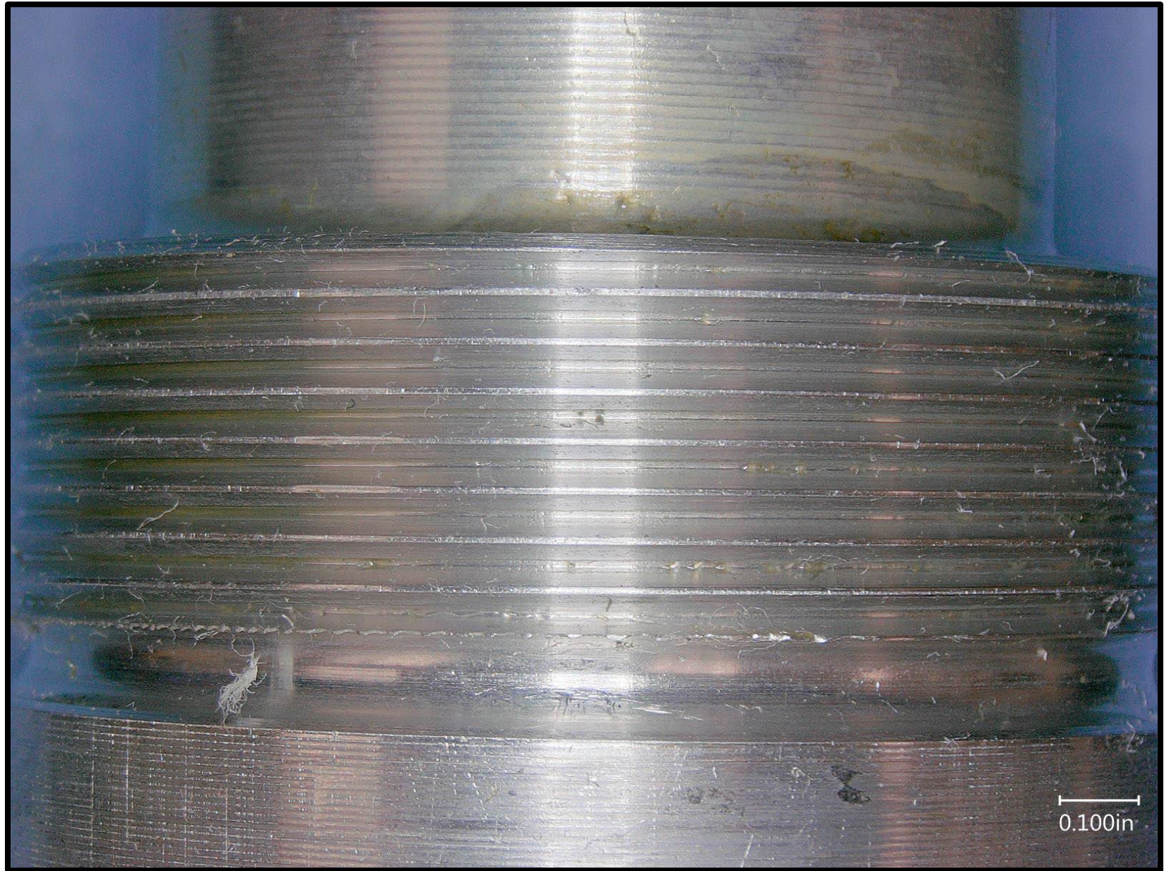
Figure 1: Hub (showing thread wear)
