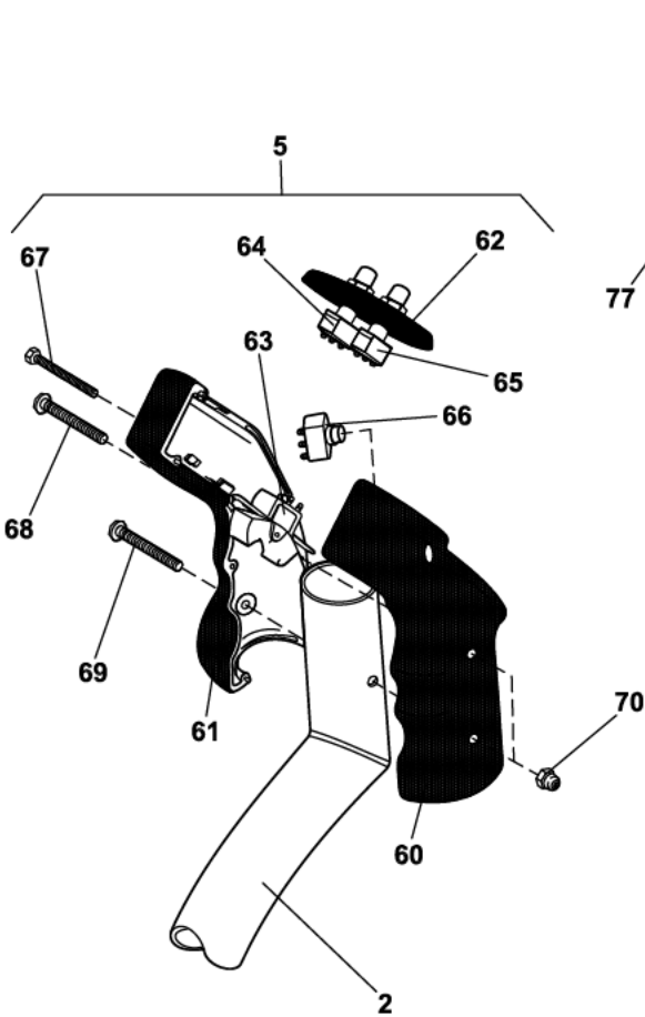
Flagger Stick Grip Assembly
