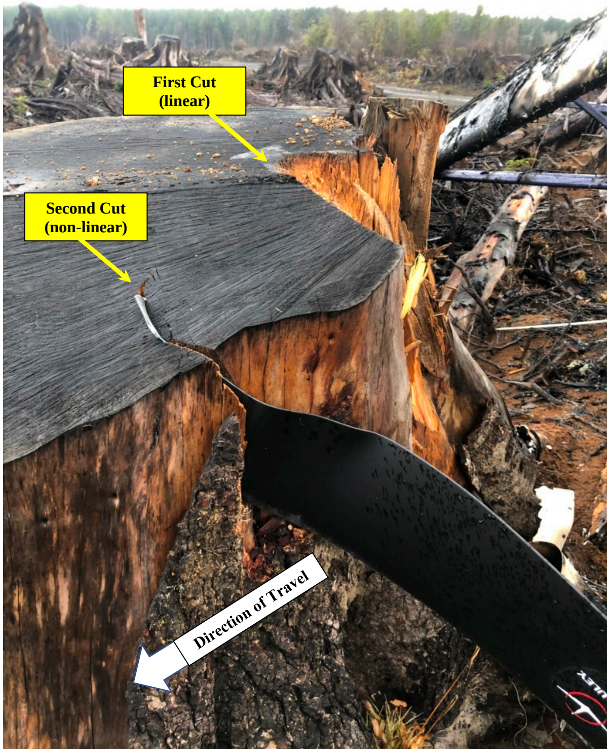
Figure 14 - Propeller Blade Cut in Stump
