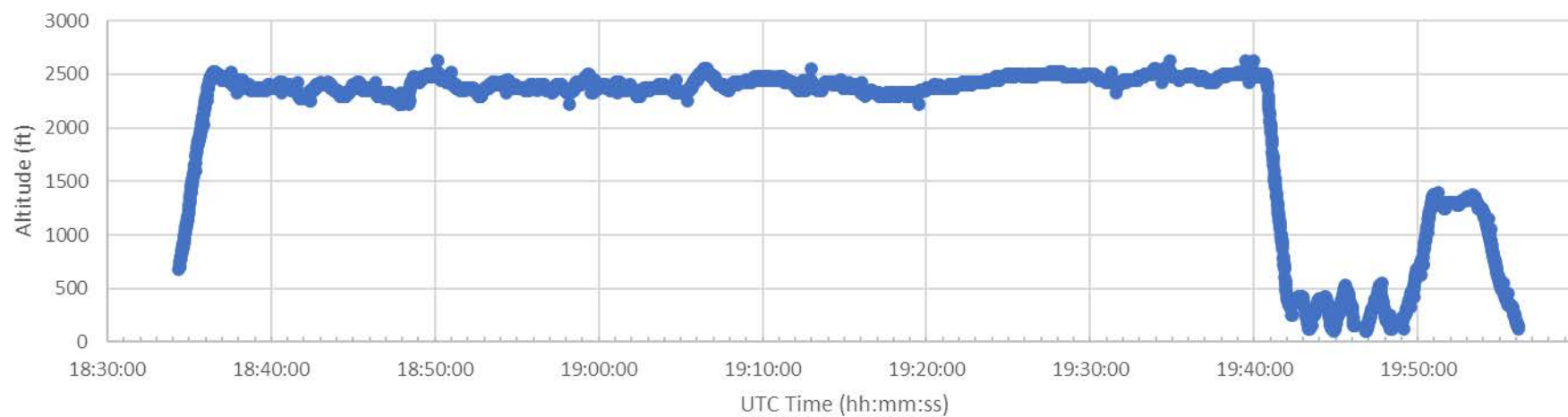
WPR19LA105 - ADS-B Altitude
