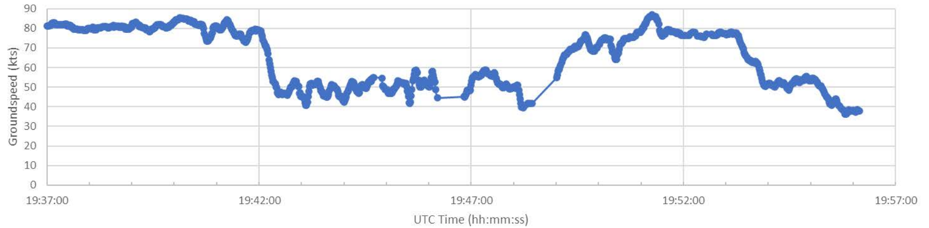
WPR19LA105 ADS-B Groundspeed
