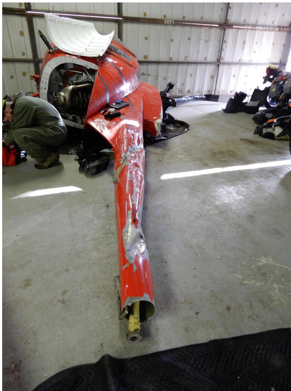
Photo 5 -View of the Tail Boom and Tail Rotor Drive Shaft
