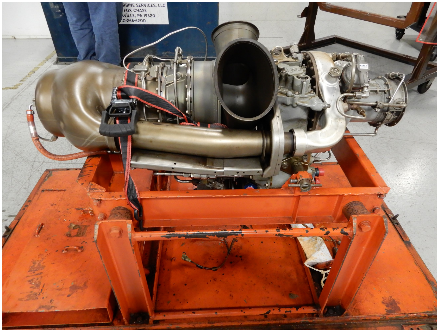
Photo 3 – Engine from N506PH, as received at the service center.
