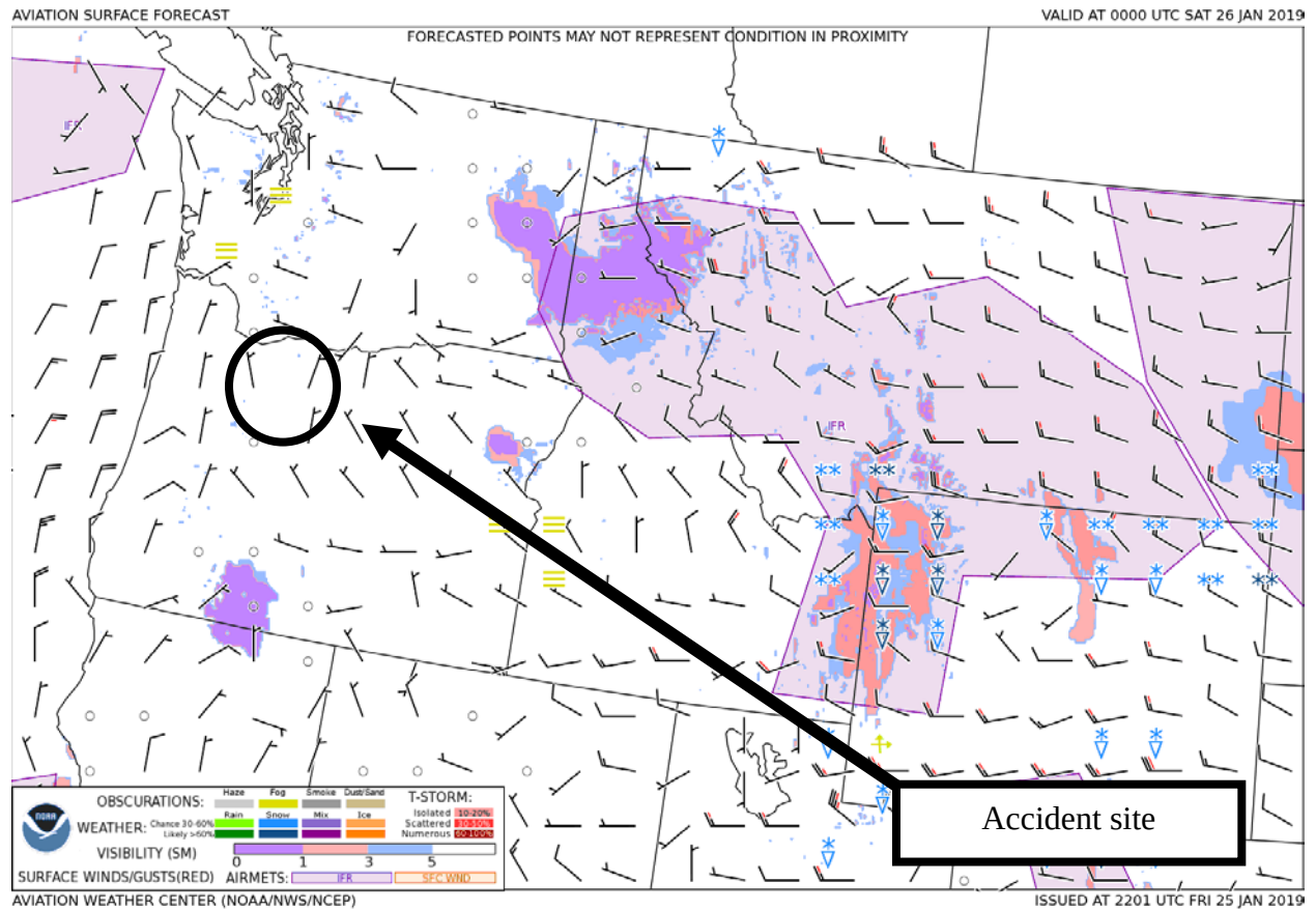
Figure 3 – GFA Surface Forecast valid at 1600 PST with forecast issued at 1401 PST
