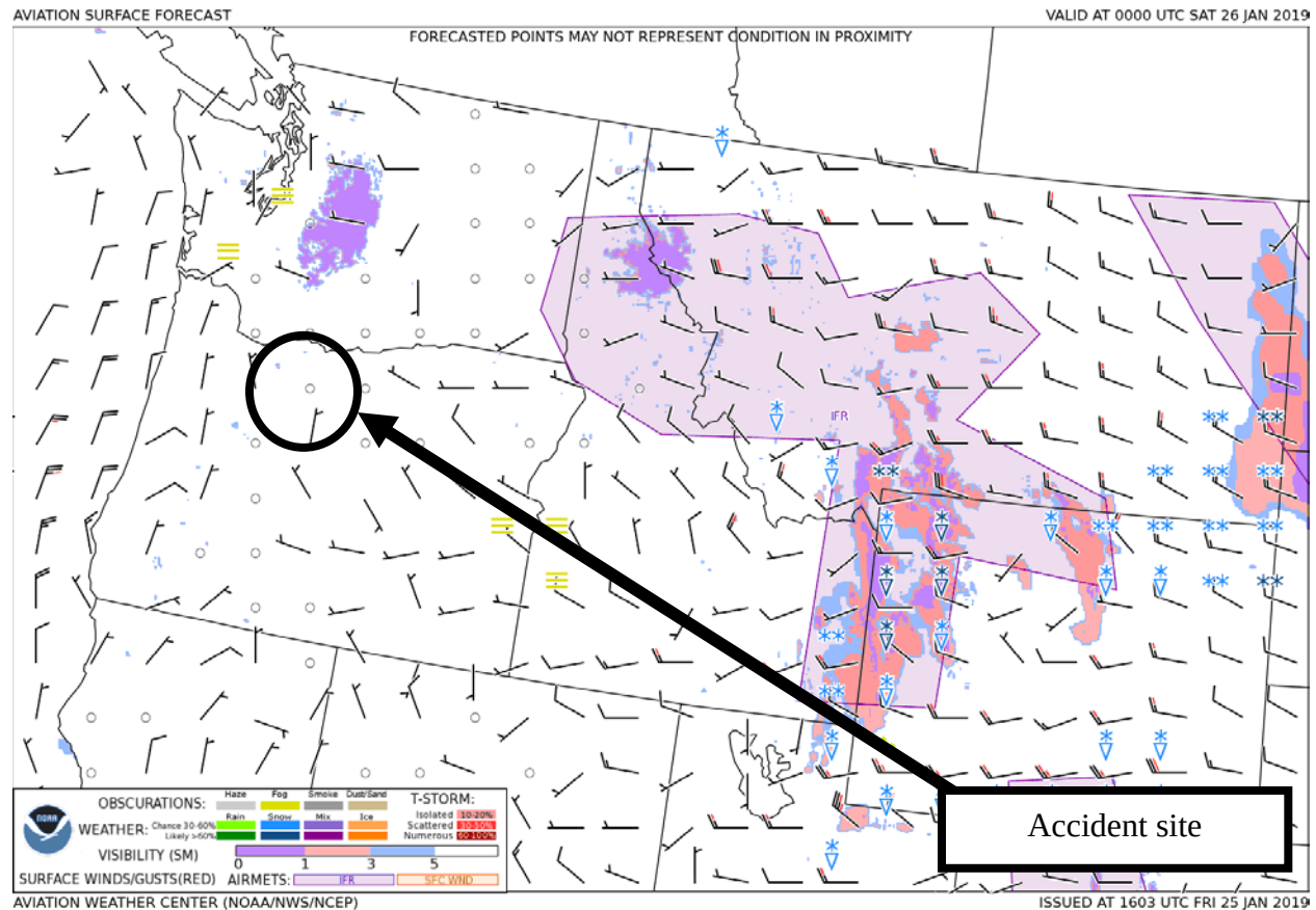
Figure 1 – GFA Surface Forecast valid at 1600 PST with forecast issued at 0803 PST
