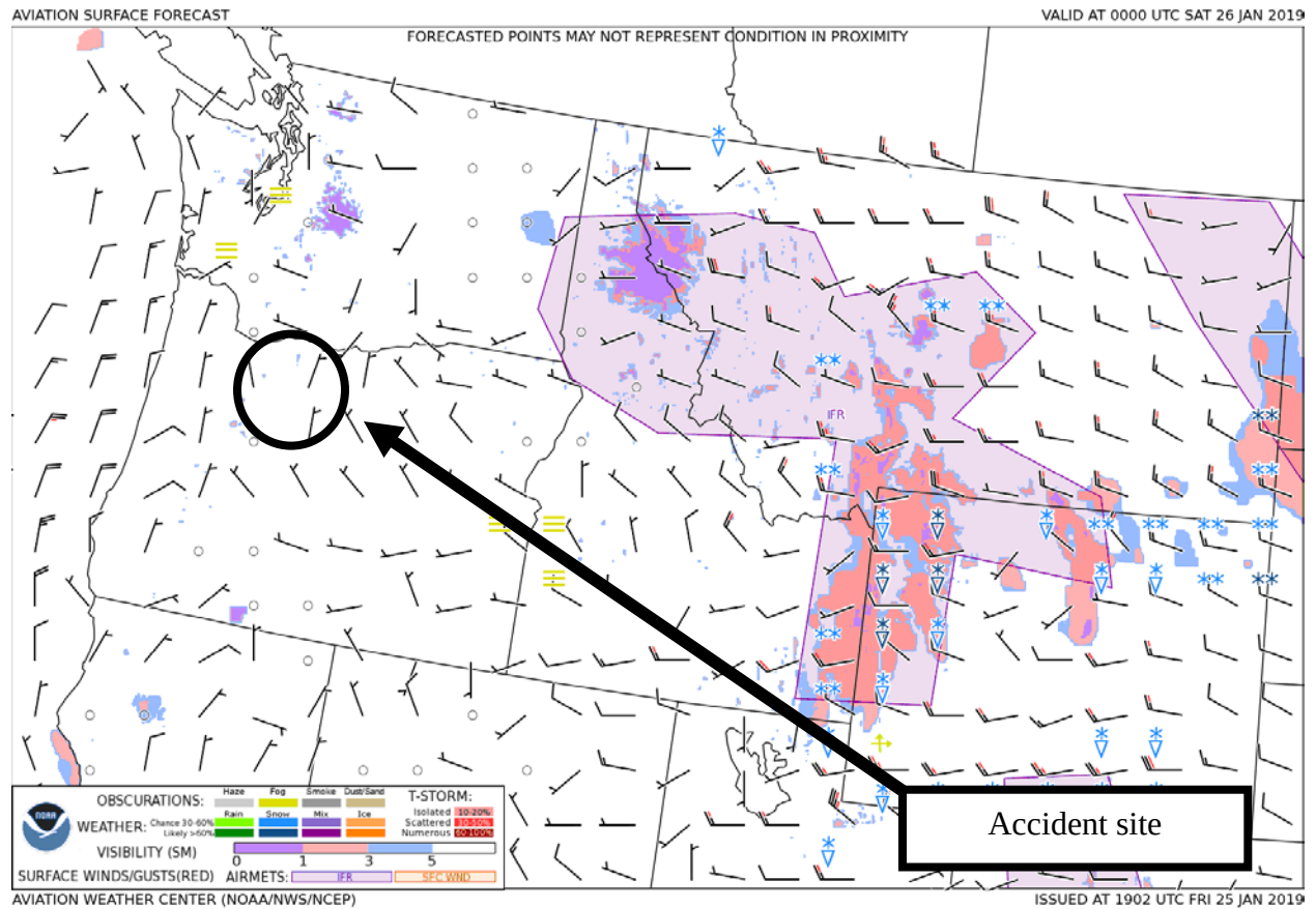
Figure 2 – GFA Surface Forecast valid at 1600 PST with forecast issued at 1102 PST
