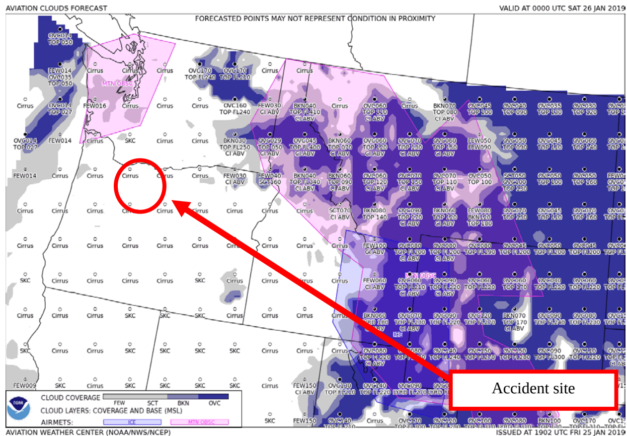
Figure 5 – GFA Aviation Clouds Forecast valid at 1600 PST with forecast issued at 1102 PST
