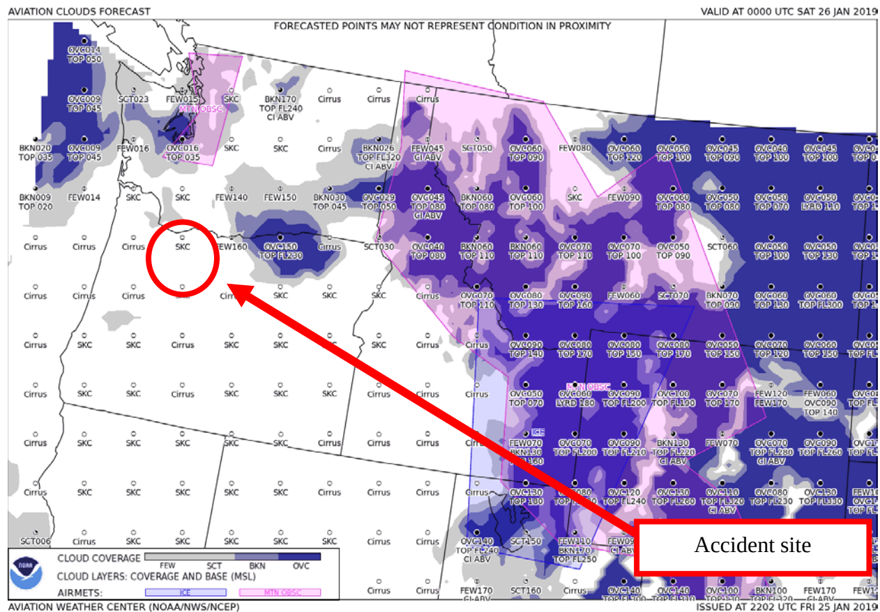
Figure 6 – GFA Aviation Clouds Forecast valid at 1600 PST with forecast issued at 1402 PST
