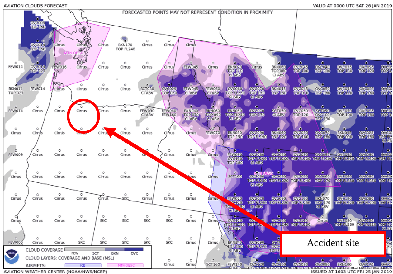
Figure 4 – GFA Aviation Clouds Forecast valid at 1600 PST with forecast issued at 0803 PST
