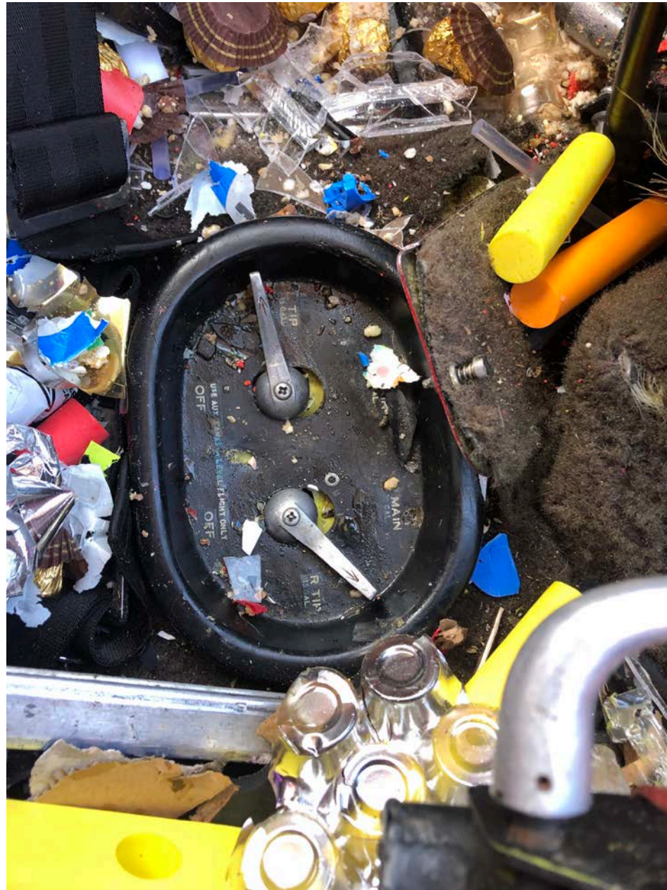
Photo 6 – View of the fuel selector valve handles.
