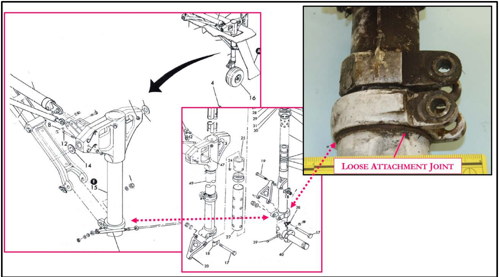
Figure 2: Failed Joint
