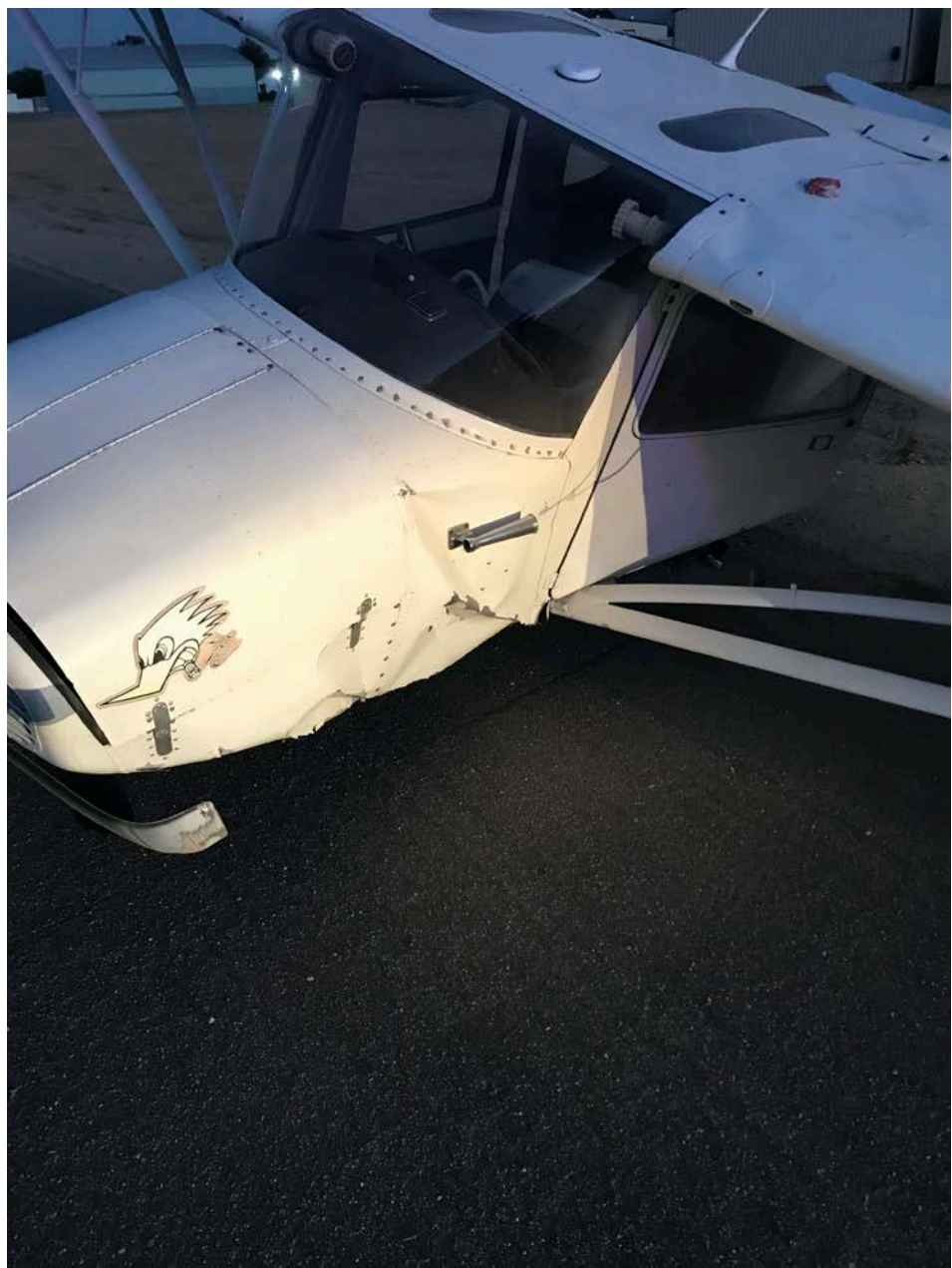
Photo 2 – Forward Fuselage
