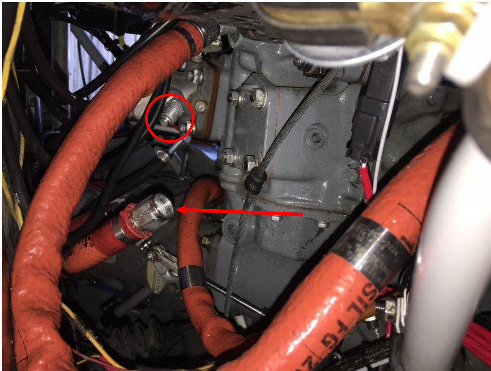
Photo 5 –Engine Accessory Case with Separated Fuel Line (Courtesy of Federal Aviation Administration)
