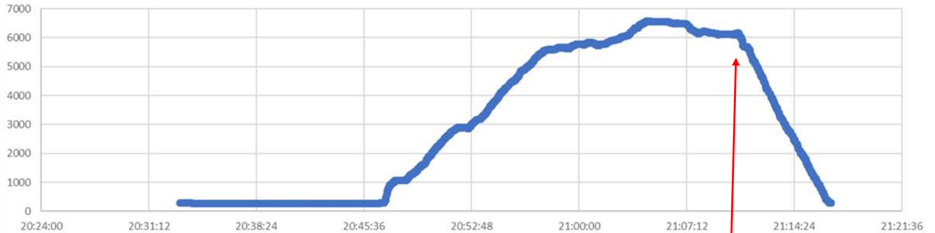
ACCIDENT FLIGHT GPS ALTITUDE
