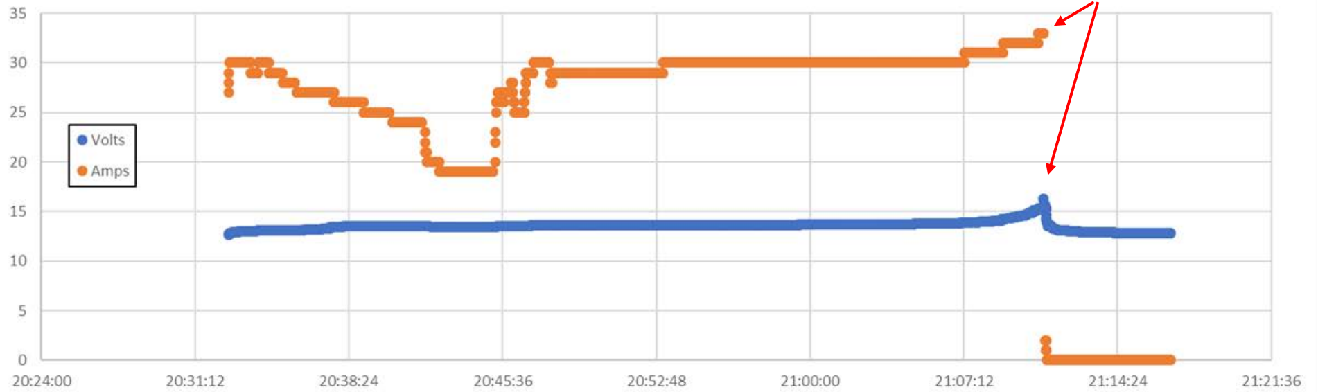
ACCIDENT FLIGHT VOLTAGE & CURRENT
