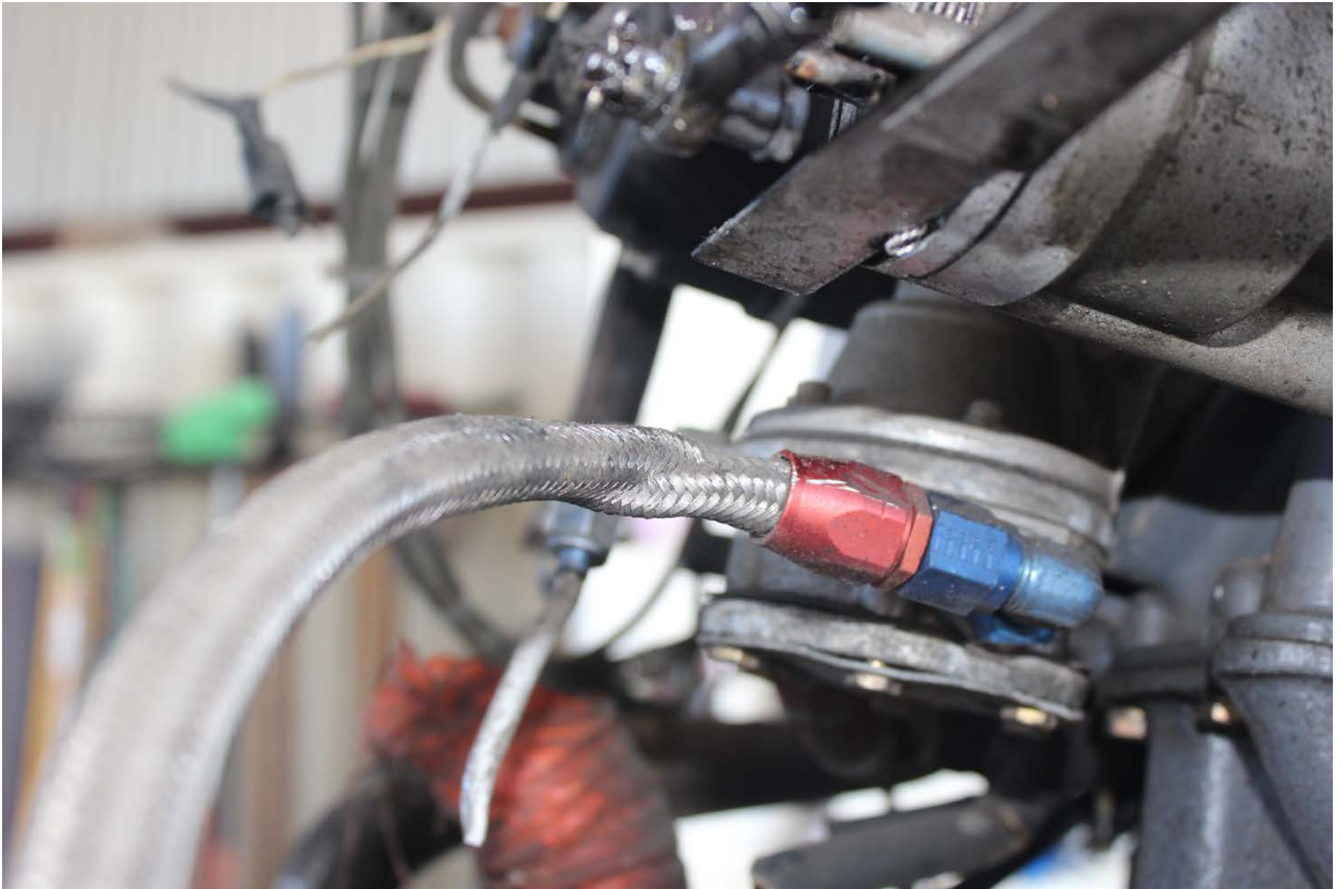
Photo 6 – N46321 Fuel Hose Showing Deformation
