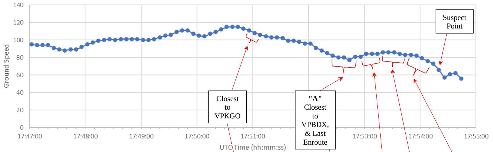
WPR18FA251 Ground Speed from JPI
