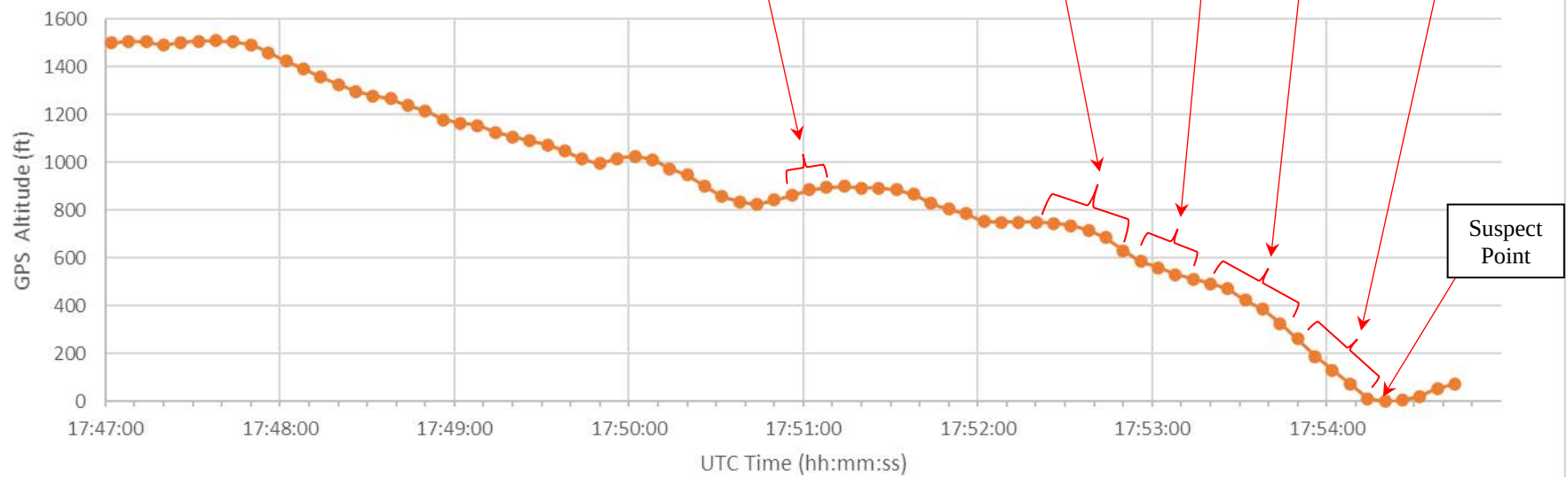
WPR18FA251 GPS Altitude from JPI
