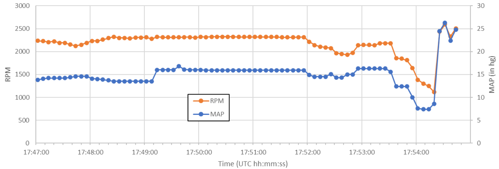
WPR18FA251 Engine Data
