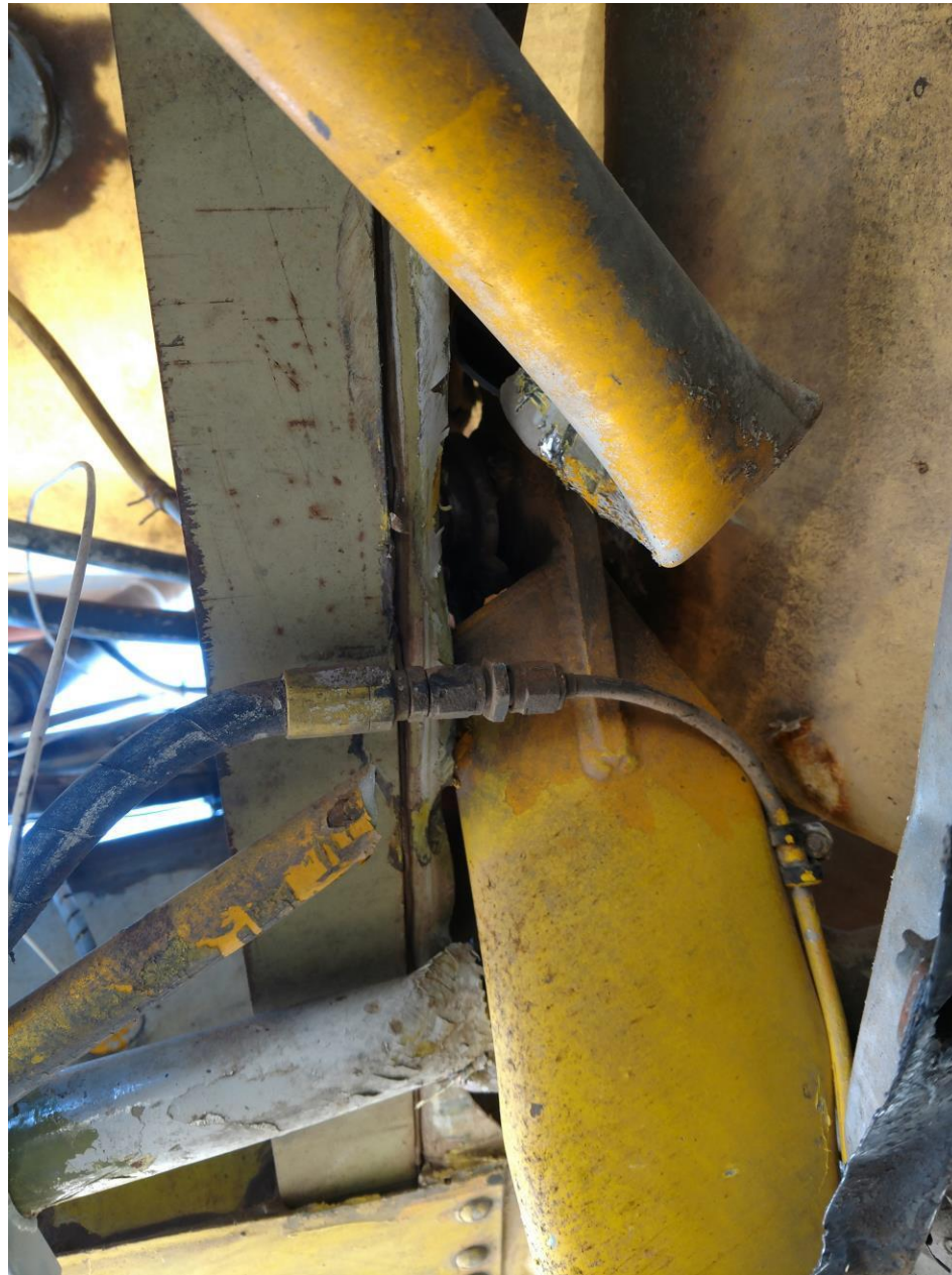
Photo 2 – Substantial damage at the fuselage to landing gear attachment
