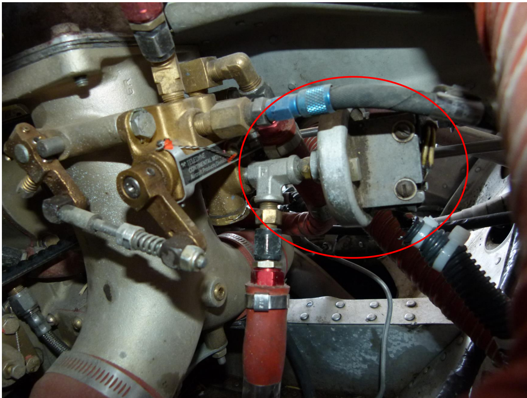
Photo 4 – Fuel pressure switch.
