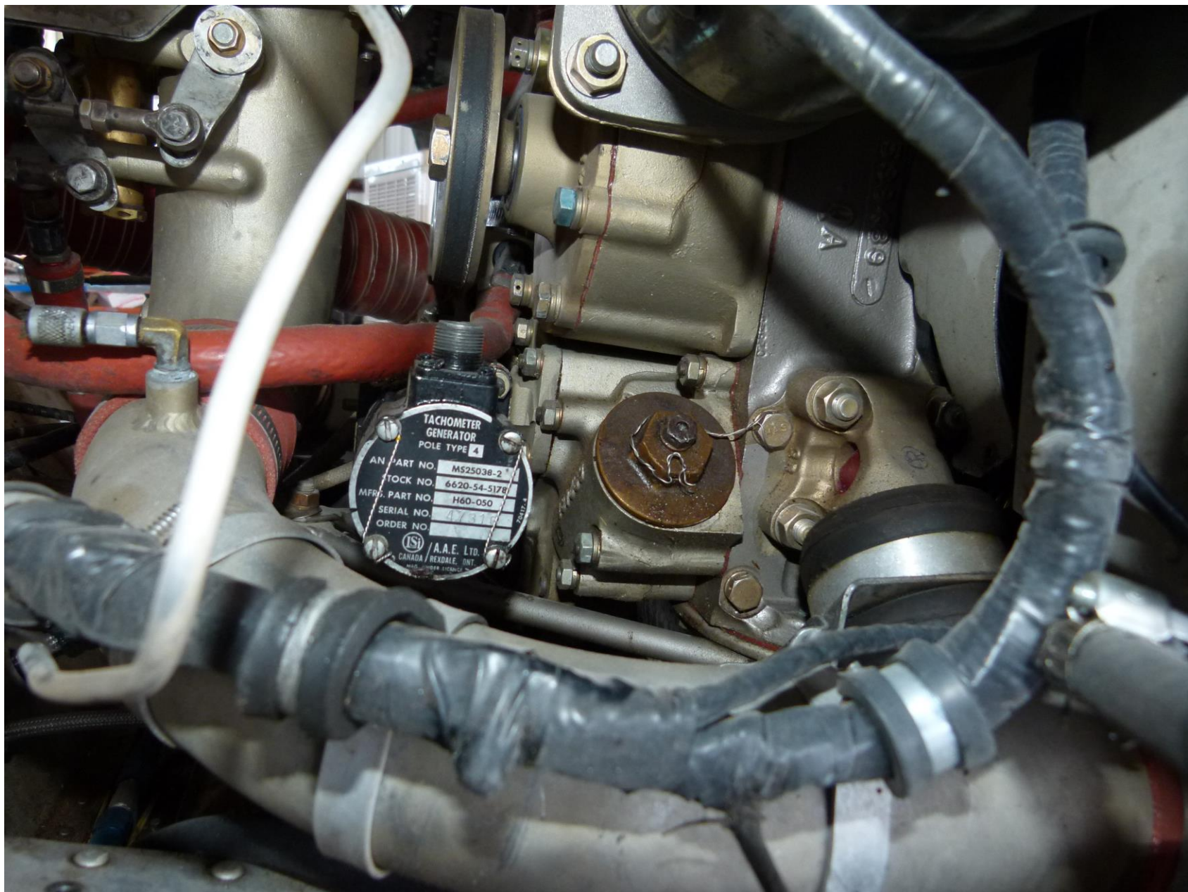
Photo 6 – Left engine tachometer generator and oil screen cap.
