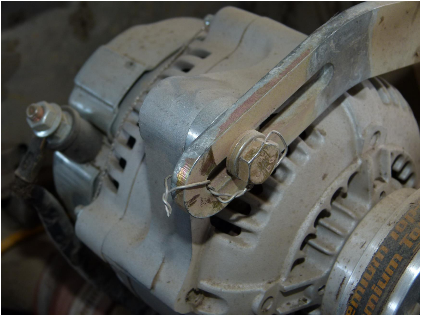
Photo 8 – Right engine belt driven alternator adjustment hardware safety wire.
