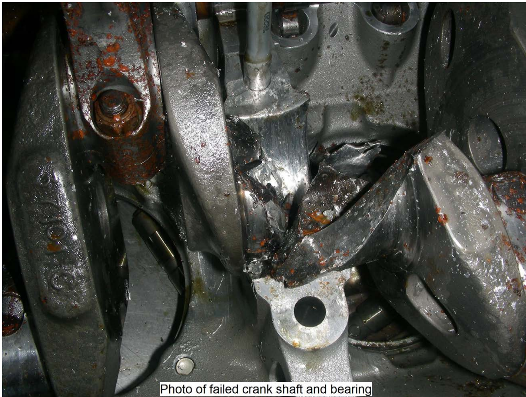
Photo 6 – photo of failed crank shaft and bearing
