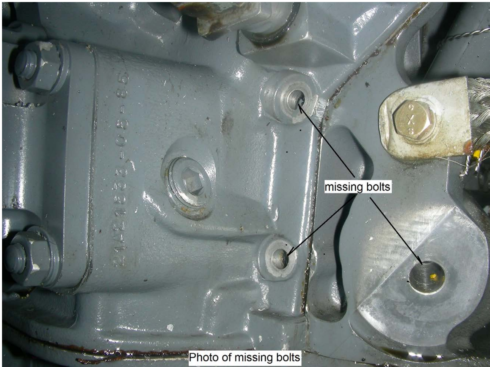
Photo 4 – photo of missing case bolts
