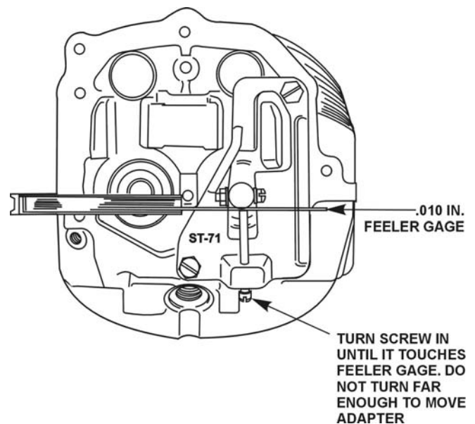
Figure 6. Feeler Gage in Position Between Set Screw and Adapter Post
