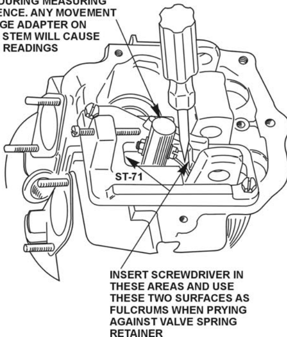
Figure 5. View Showing Screwdriver in Position to Move Exhaust Valve Stem
