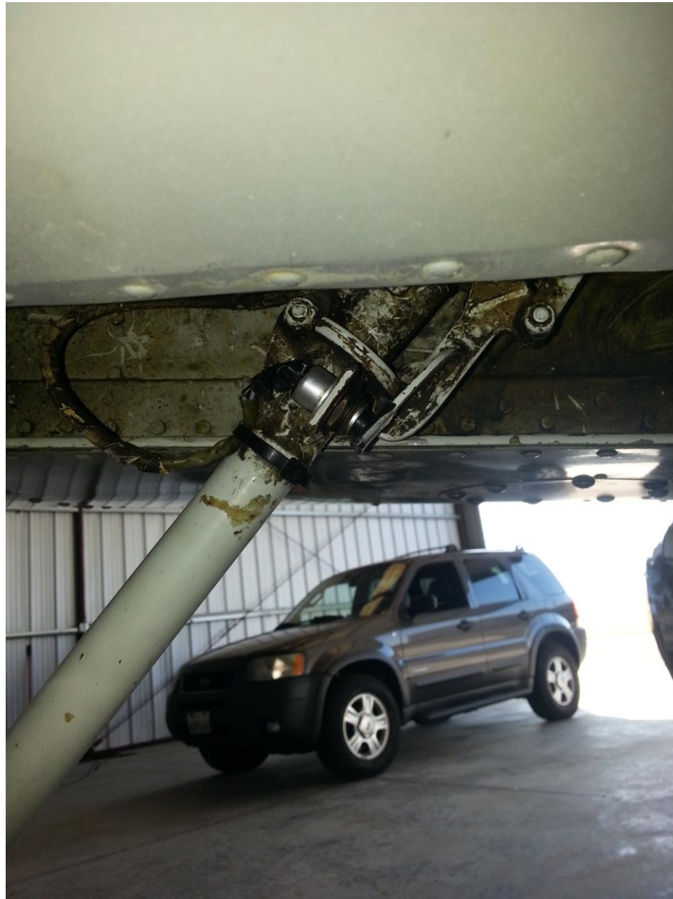
Photo 5 – Left main landing gear position switch.
