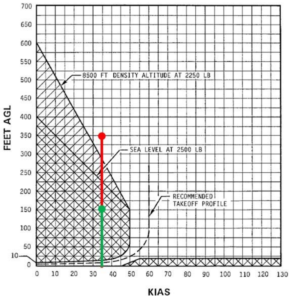
HEIGHT - VELOCITY DIAGRAM
