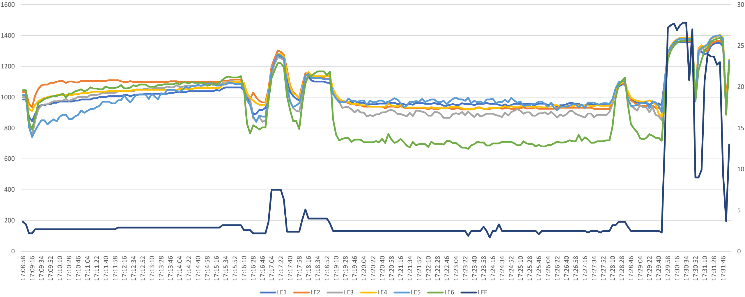
Left Engine EGT & FF
