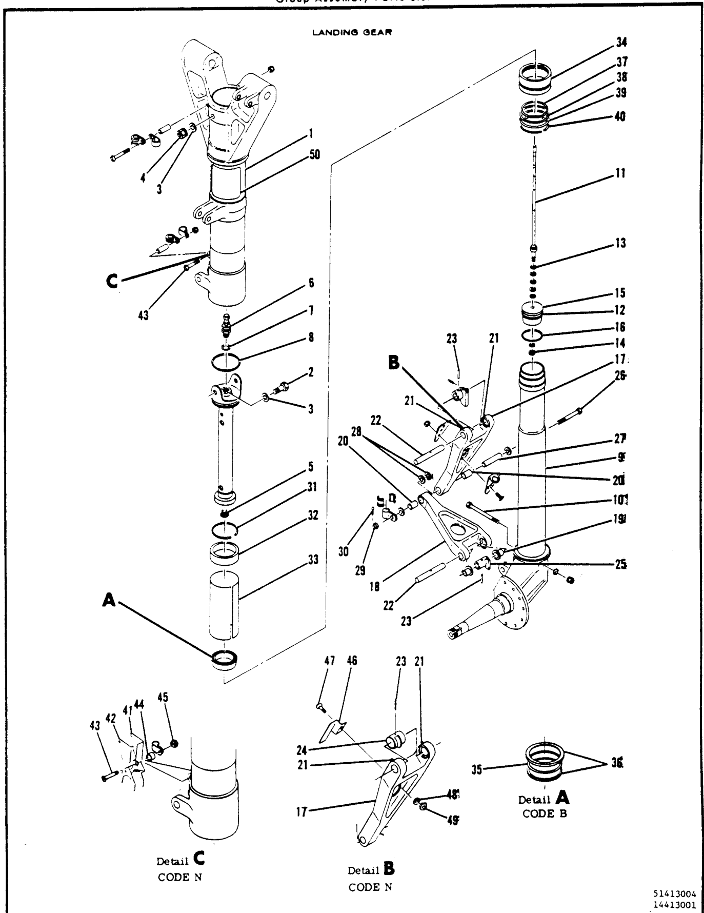
Figure 102. Main Gear Strut Installation
