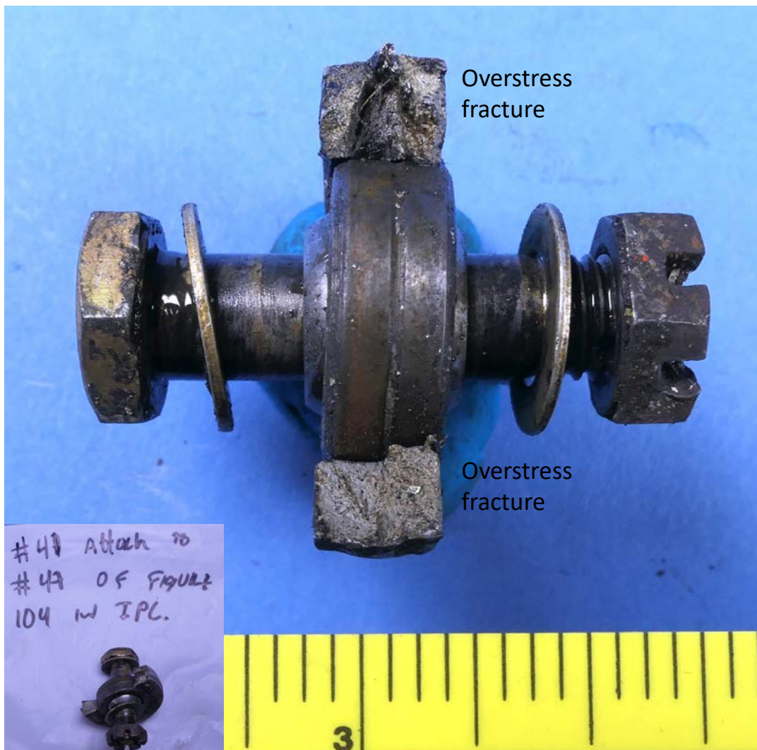
Fractured portion of swivel bearing assembly
