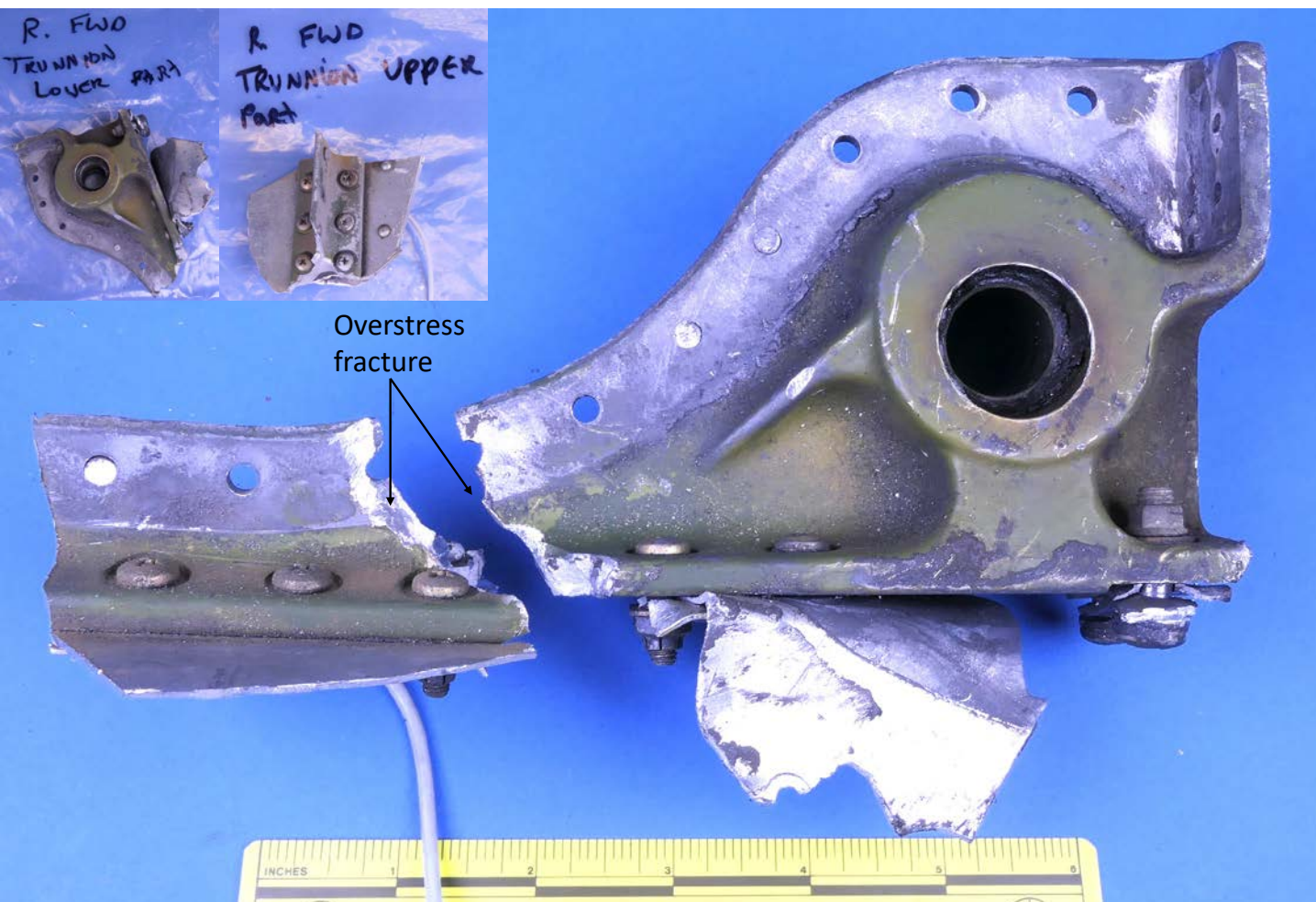
Pieces of fractured trunnion
