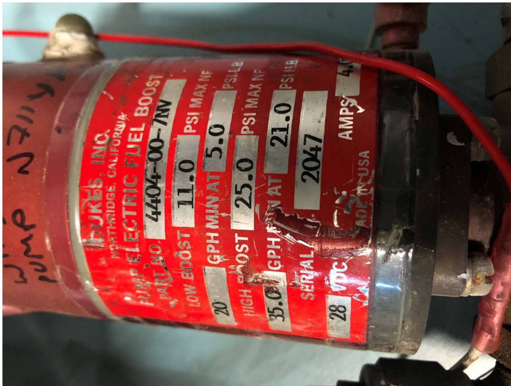
Photo 1 – Left wing fuel pump as removed.
