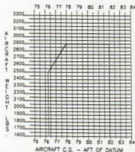
EXPRESS FT RECOMENDED CENTER OF GRAVITY LIMITS EXPRESS DESIGN INC. DATE 02-14-95
