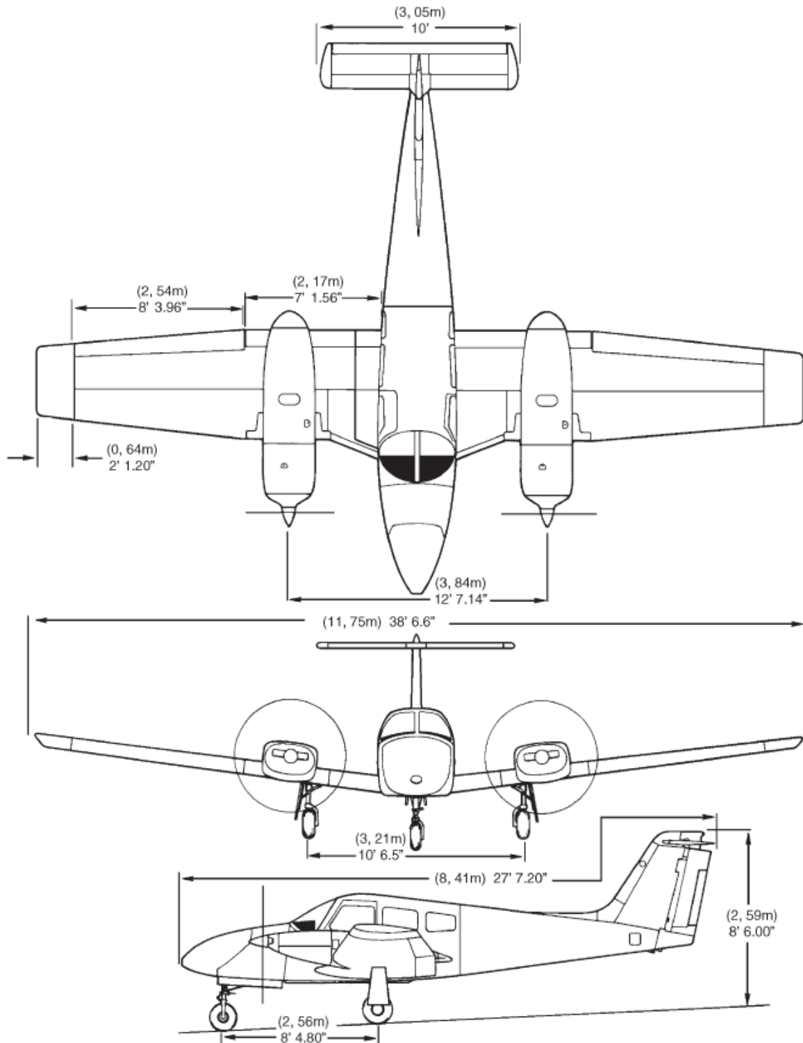
Figure 1 – Piper PA-44-180 3-view drawing
