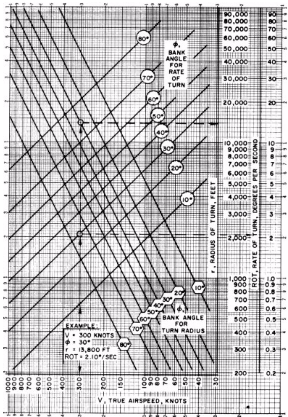
Figure 2.29. General Turning Performance (Constant Altitude, Steady Turn)
