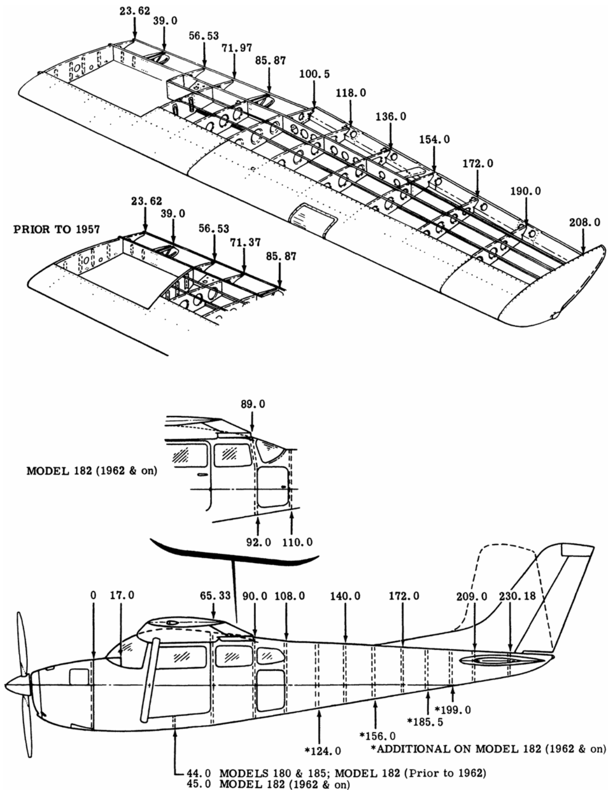
Figure 2 – Cessna 180 wing and fuselage station diagram
