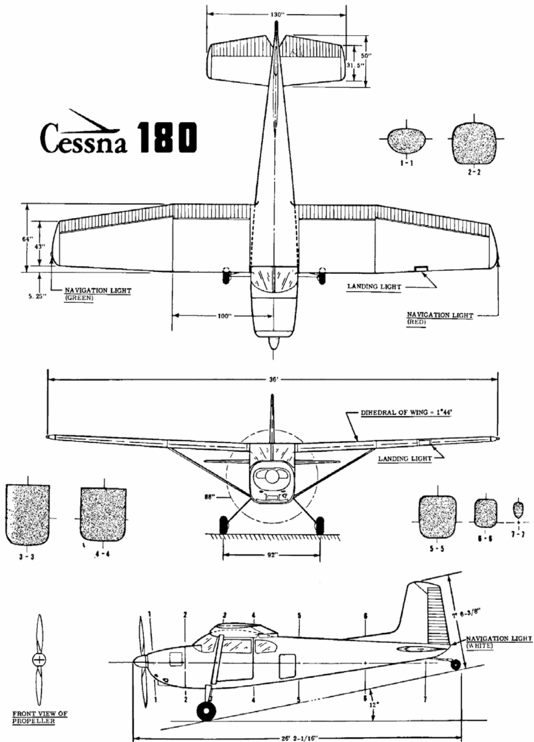
Figure 1 – Cessna 180 3-view drawing
