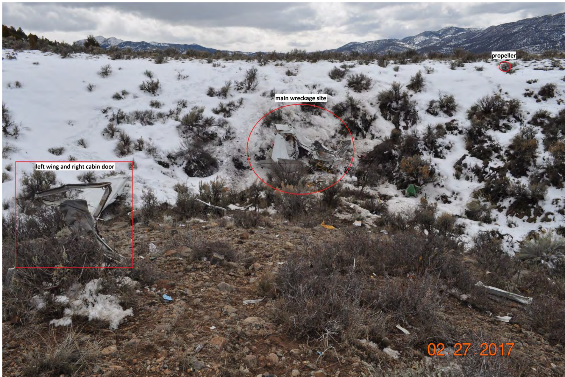
Photo 2 – view of main wreckage site looking southwest
