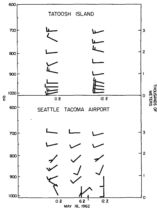
FIG. 11. Vertical soundings at Seattle-Tacoma airport and Tatoosh Island during the convergence event of 18 May 1962. The arrow indicates the time of convergence zone passage.
