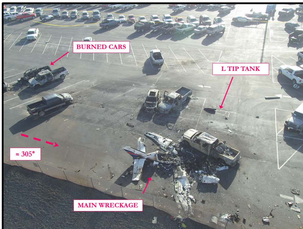
Figure 3: Main Wreckage
