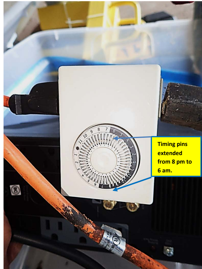
Photo 13-Mechanical pin timer for vertical hangar lights
