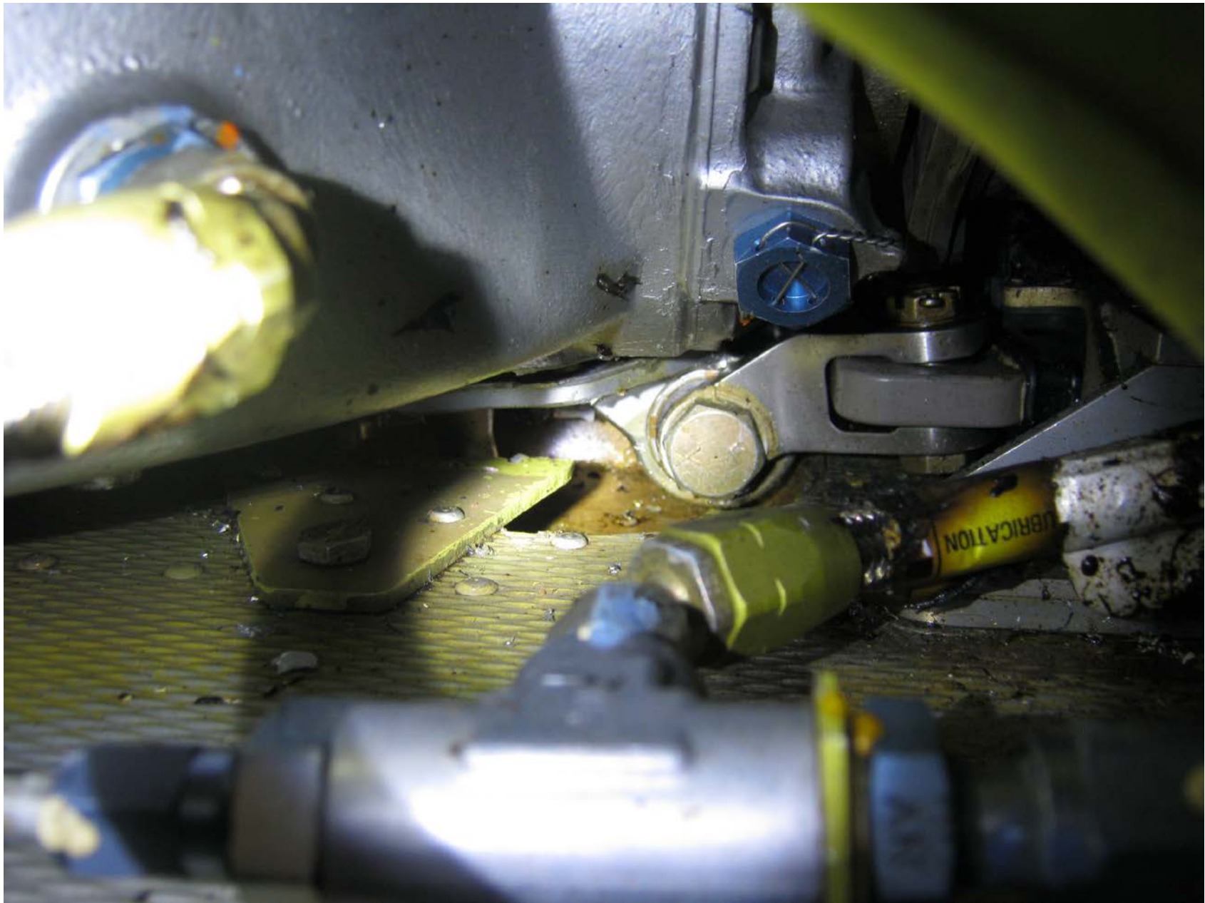
Photo 6 – View of lower transmission housing (courtesy of the Department of Interior)
