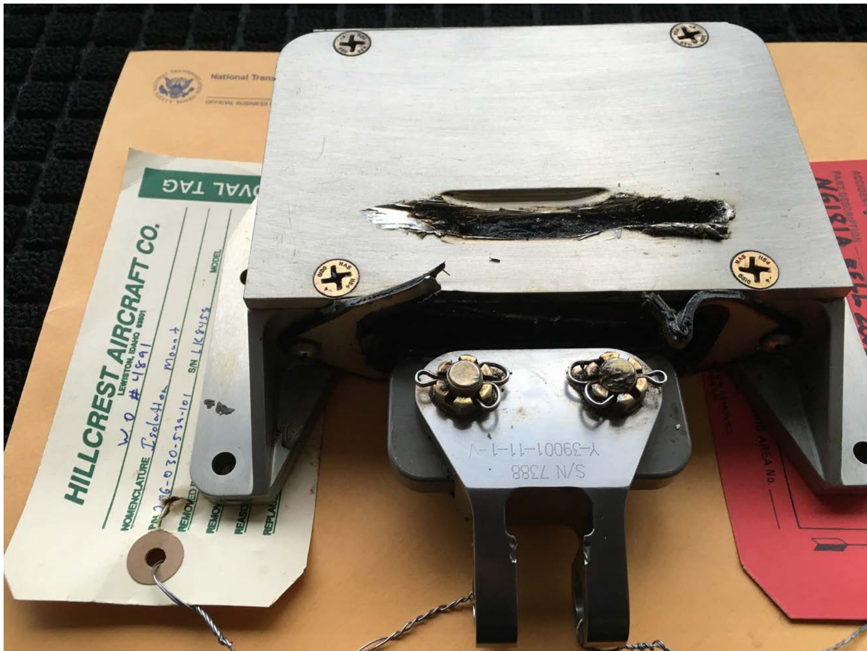
Photo 8 – View of pylon mount (courtesy of the NTSB)
