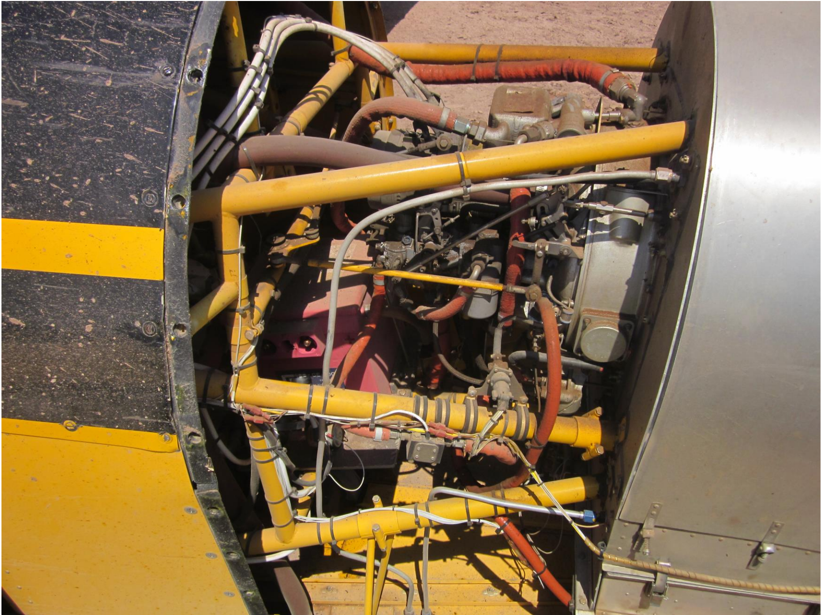
Photo 8 – Rear Engine Area and Engine Mounting Assembly
