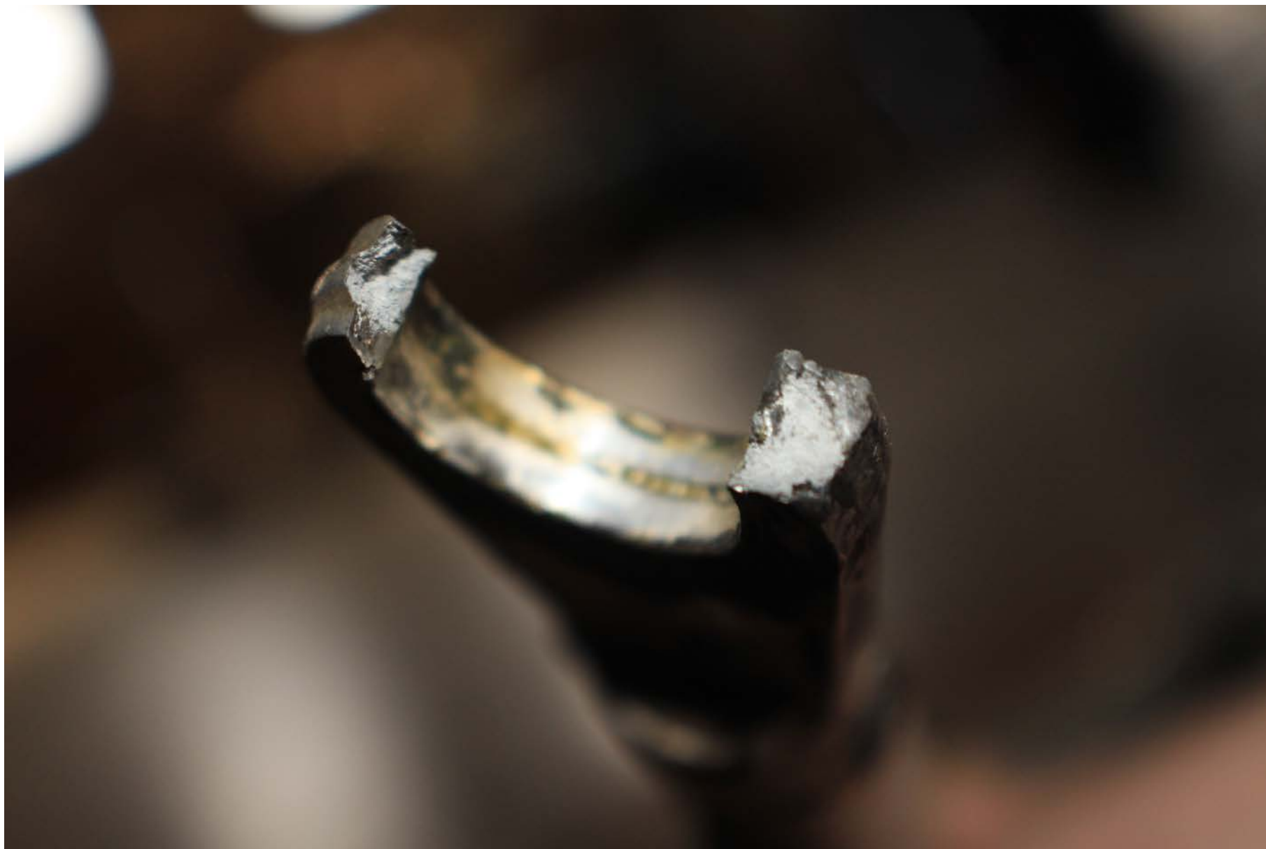
Photo 4 – Right Main Landing Gear Rod End
