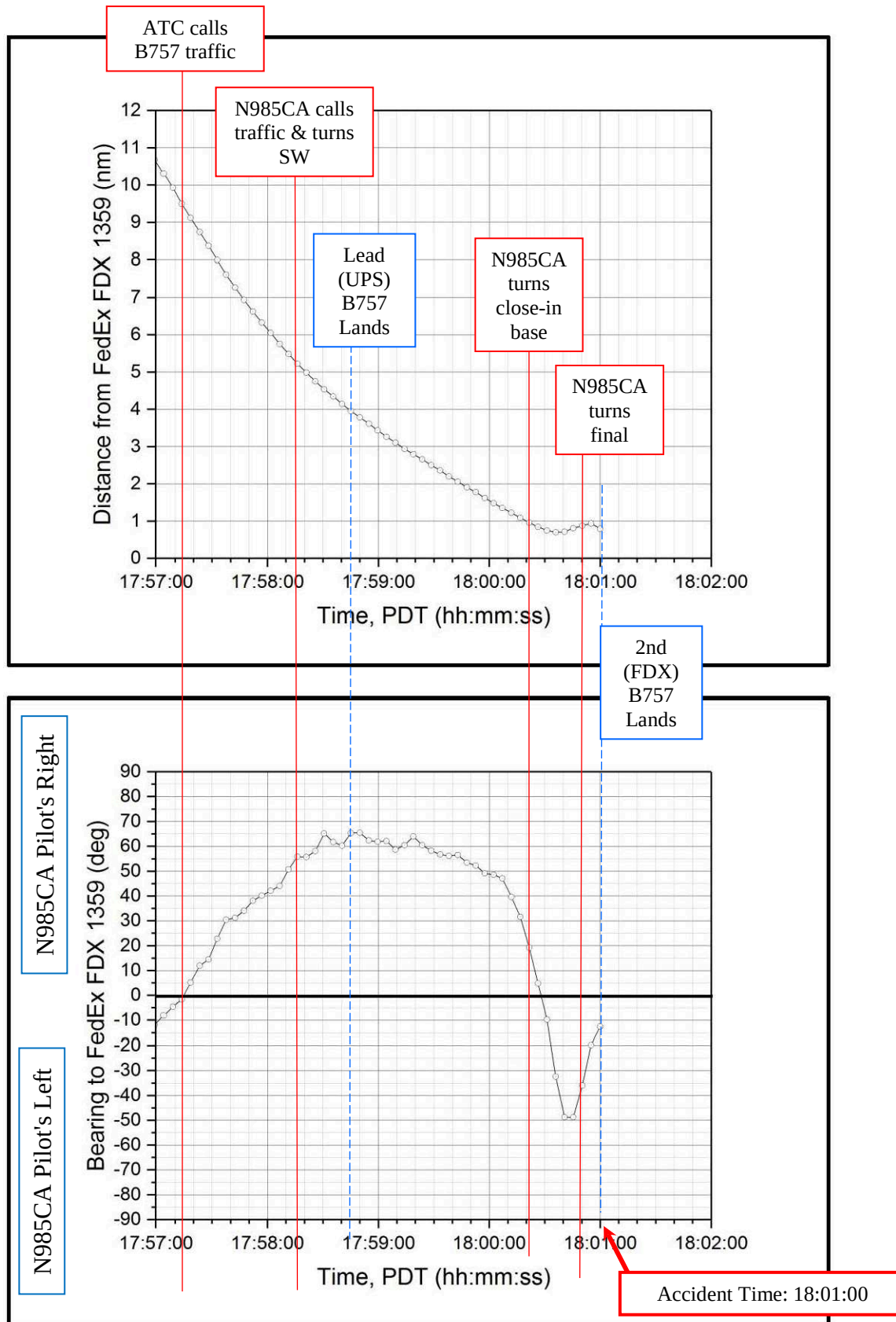
Figure 7: Distance and Bearing from N985CA to FDX1389
