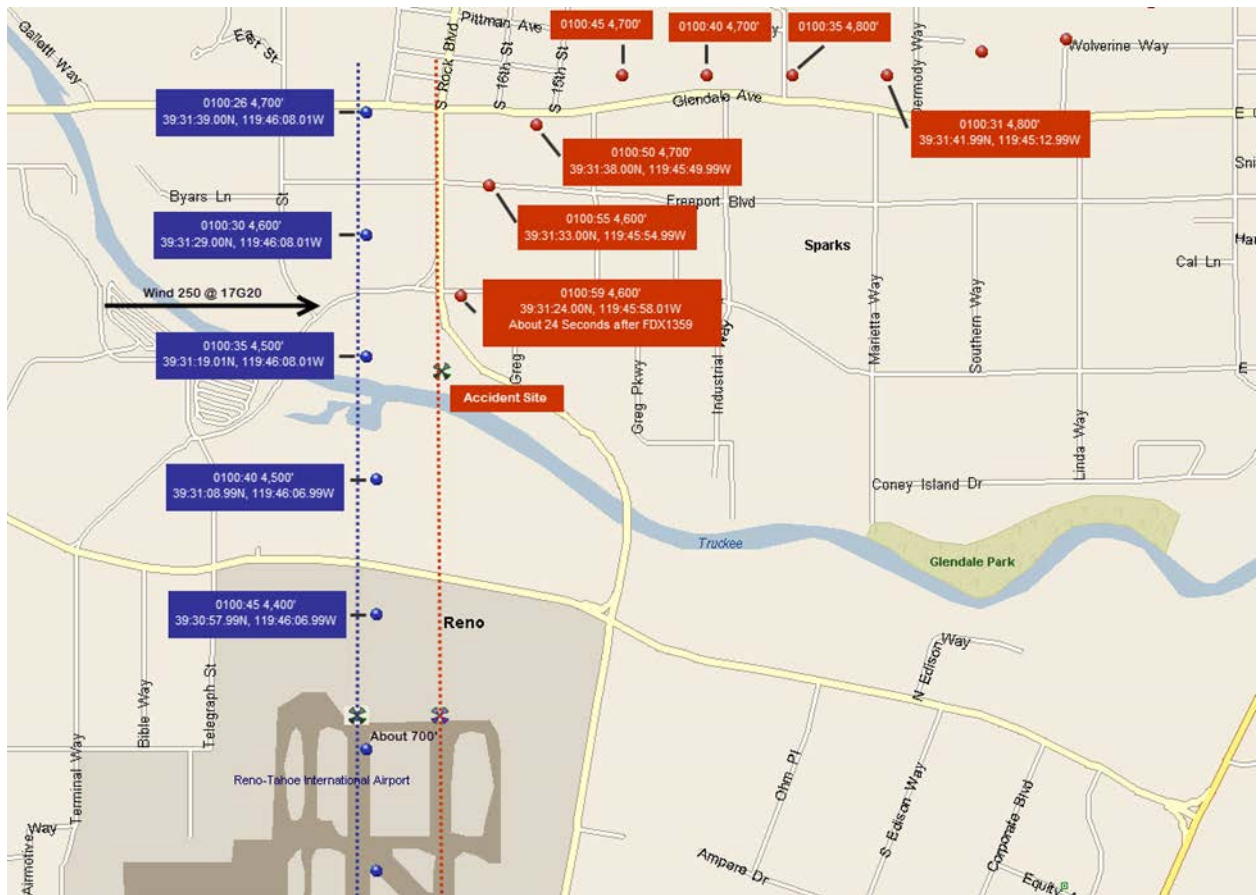
Figure 3 - Close in of the final radar plot of flight path in relation to the radar plot of the flight path of FDX1359.
