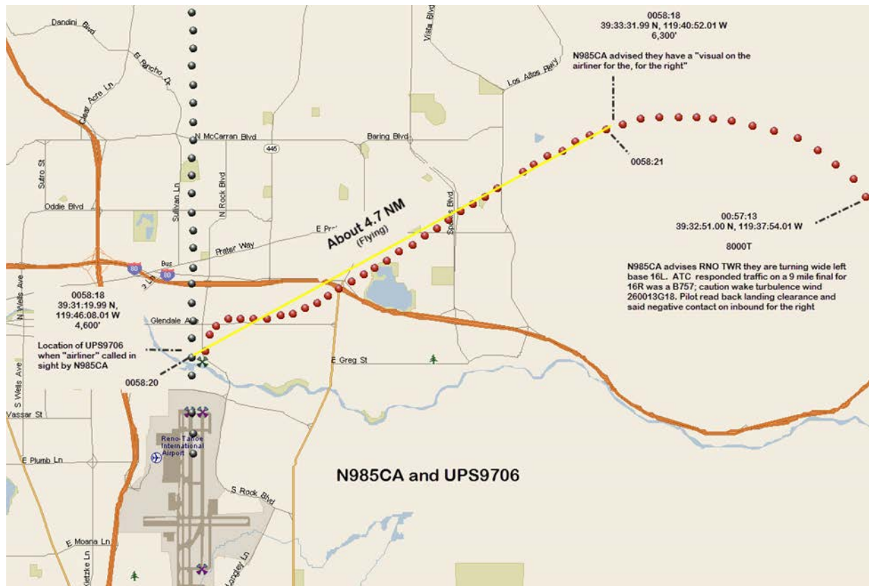
Figure 2 - Graphic showing N985CA radar plot of flight path in relation to the radar plot of the flight path of UPS9706.
