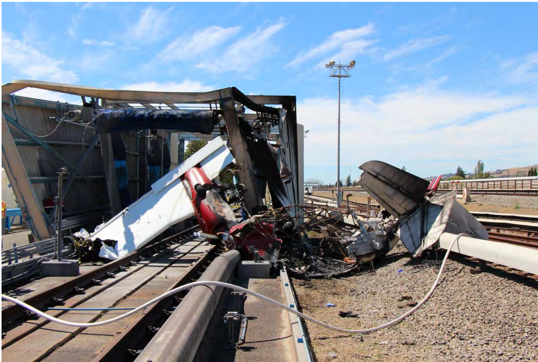
Photo 1 – View to Northwest of Aircraft at Accident Site
