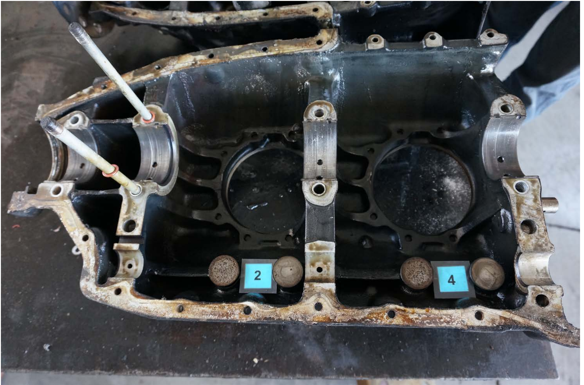
Photo 5 – Engine case half displaying main bearing scoring and spalling of intake valve tappet faces
