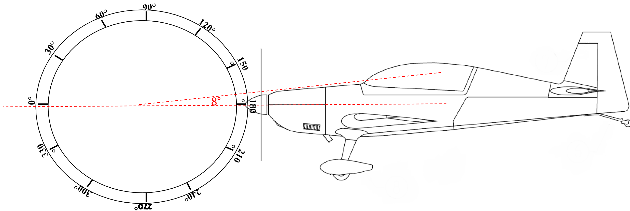
Figure 2: Airplane diagram from a left side view and estimated forward downward visibility limitations from the back seat. (Diagram courtesy of EA-300L airplane manufacturer).
