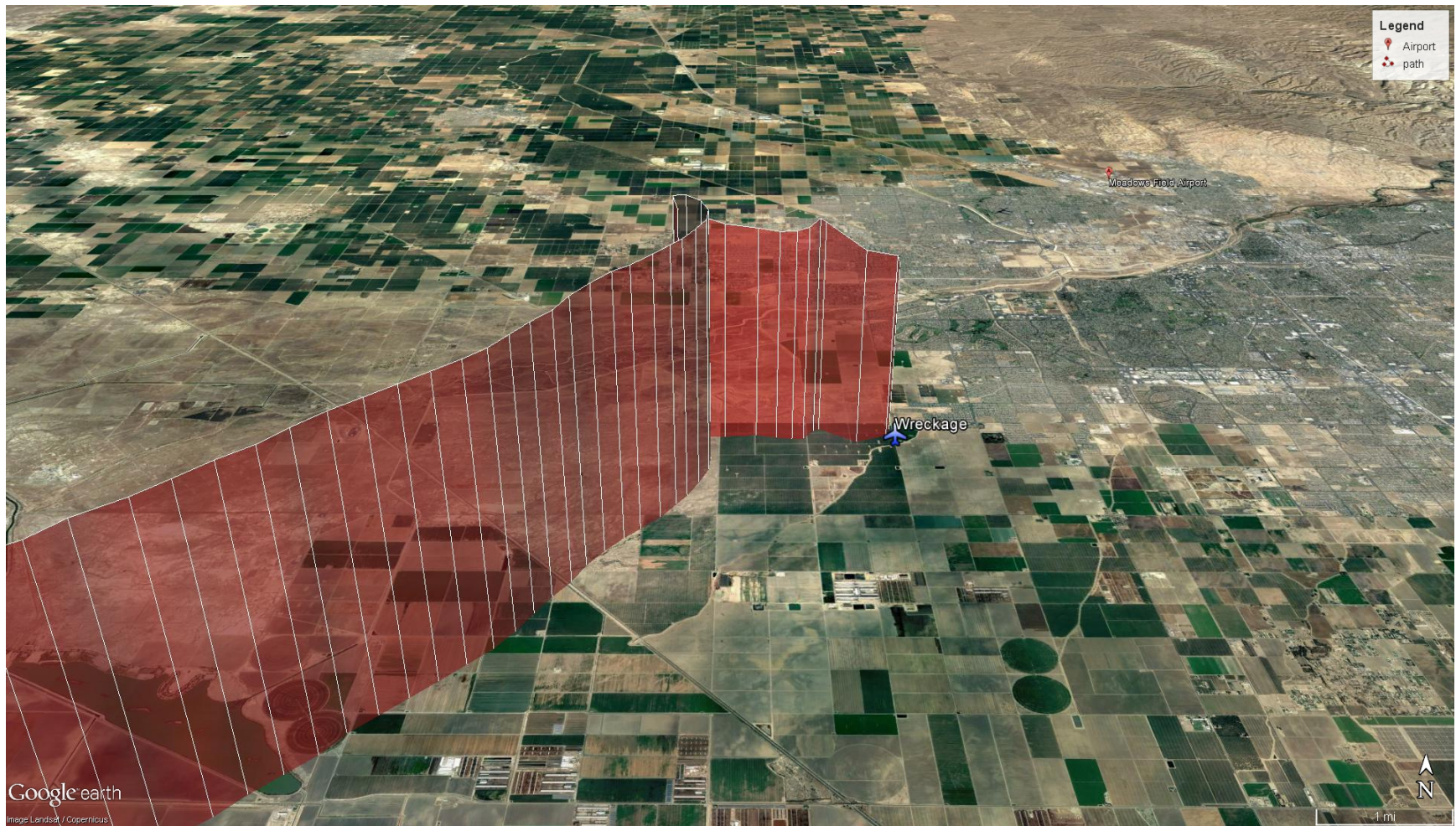
Plot 4: Final Flight Path and Wreckage Location
