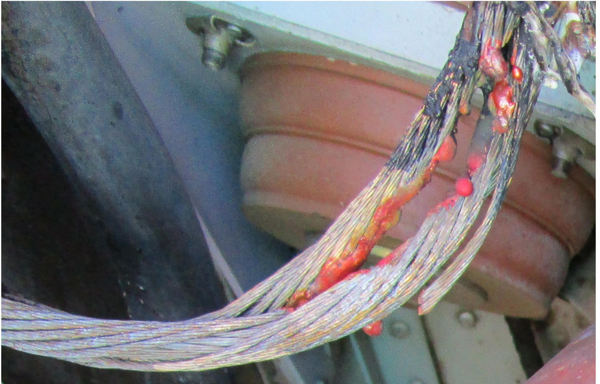
Photo 4 - Battery Cables
