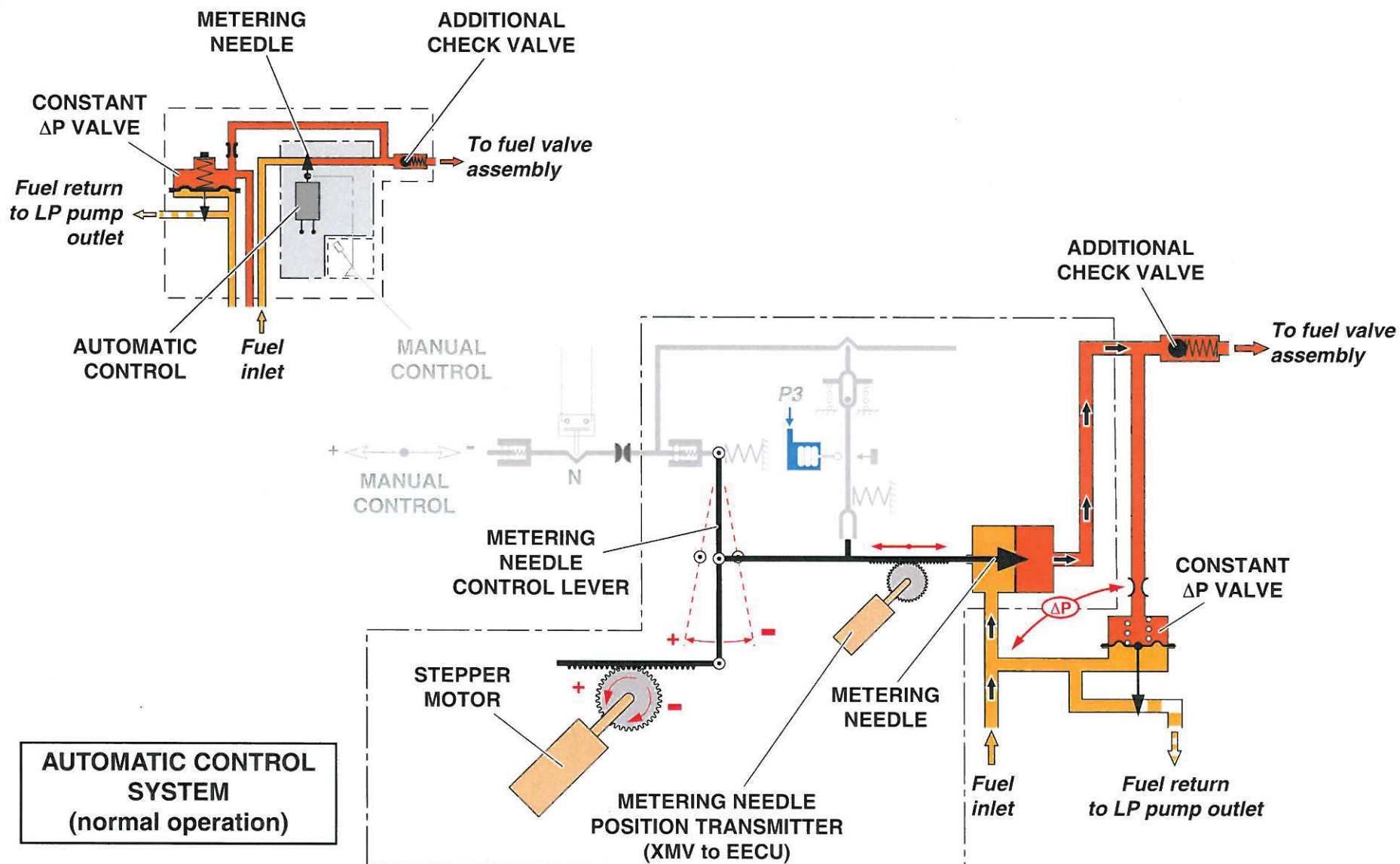
METERING UNIT (2B) - OPERATION (1) PUMP AND METERING UNIT ASSEMBLY
