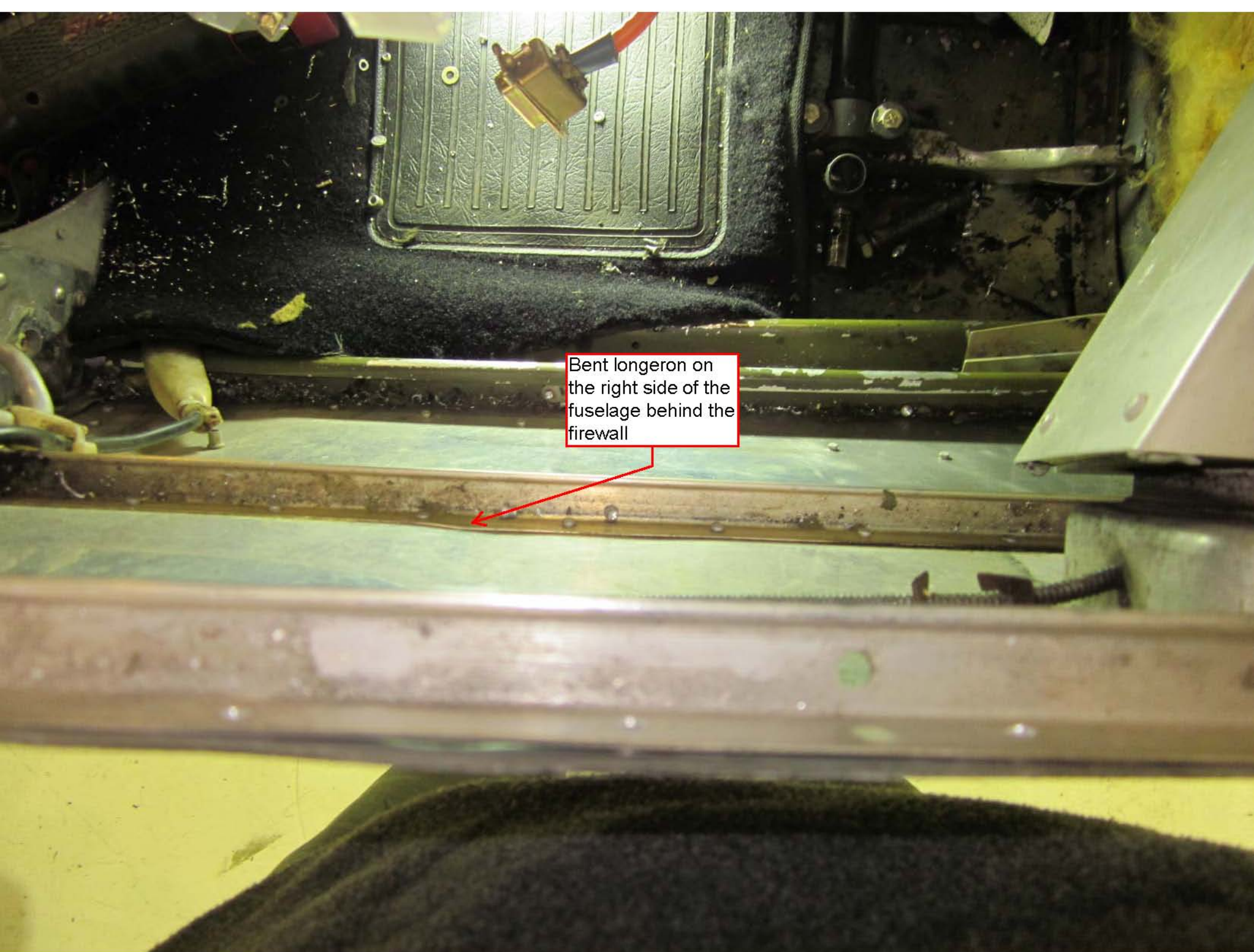
Photo 4. Bent Longeron Right Side (Provided by FAA)
