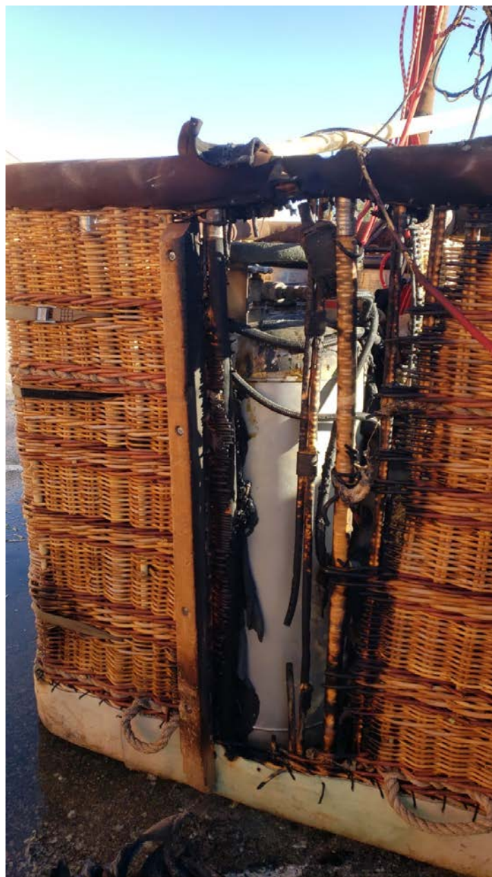
Photo 2 – View of damage to the basket (Courtesy of FAA)
