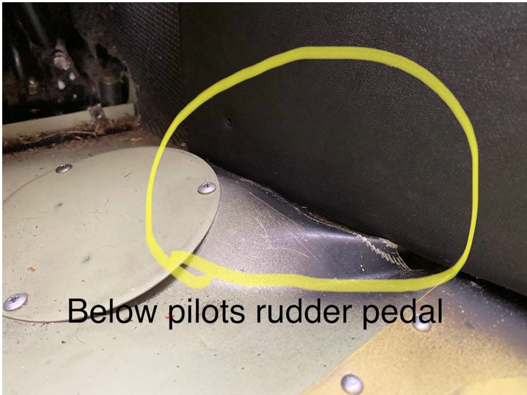
Photo 3 - View of fuselage damage (photo courtesy of the FAA)
