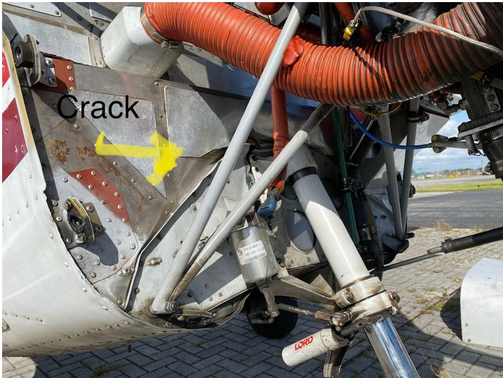
Photo 2 - View of firewall damage (photo courtesy of the FAA)
