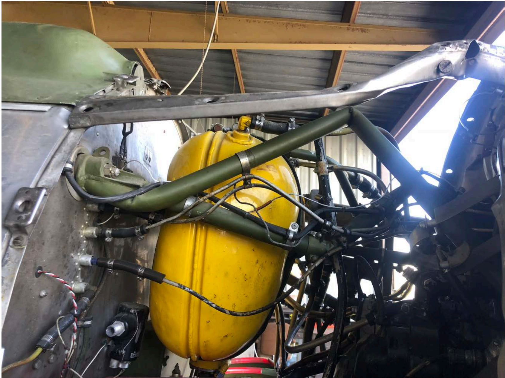
Photo – View of damaged engine mount and truss (courtesy of the FAA)
