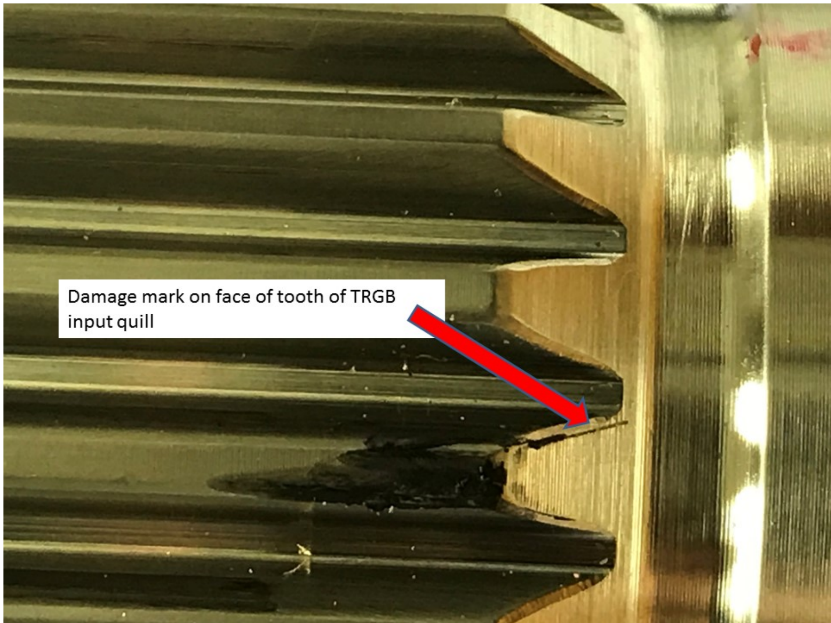
Photo 1 – View of tail rotor gear box damage (photo courtesy of the operator)
