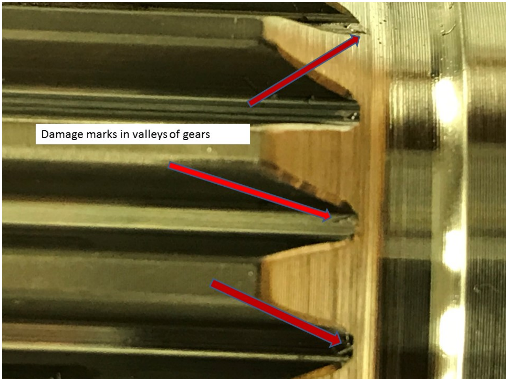
Photo 2 - View of tail rotor gear box damage (photo courtesy of the operator)
